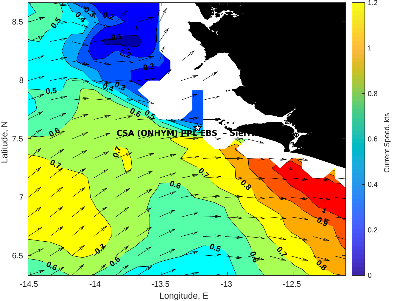
Surface Currents for CSA (ONHYM) PPL EBS - Sierra Leone at 05-Aug-2025 00:00:00
