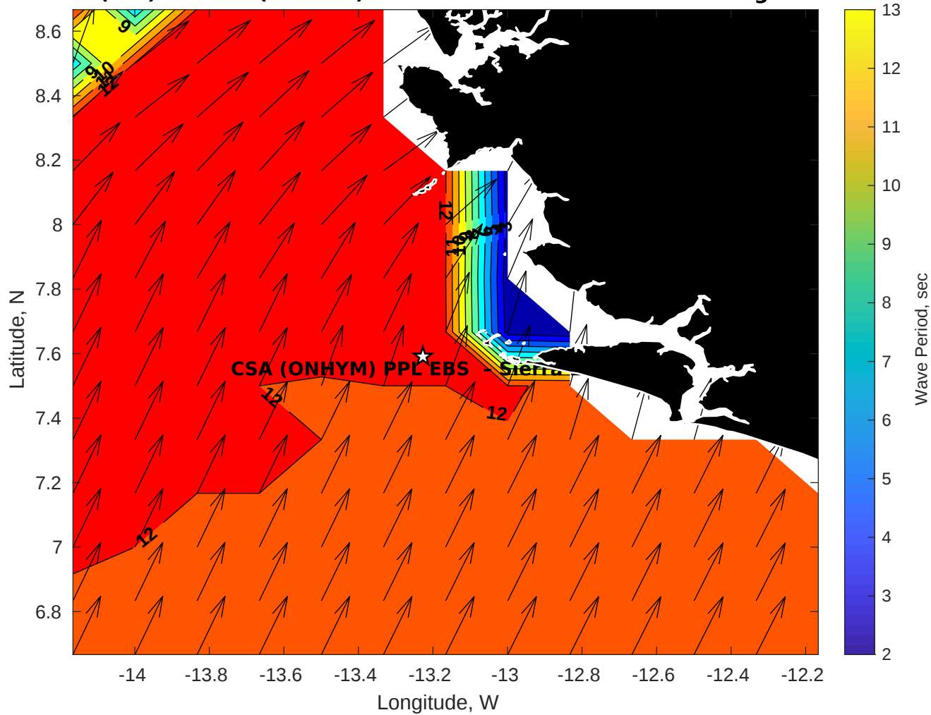
Wave Period (sec) for CSA (ONHYM) PPL EBS - Sierra Leone at 06-Aug-2025 09:00:00
