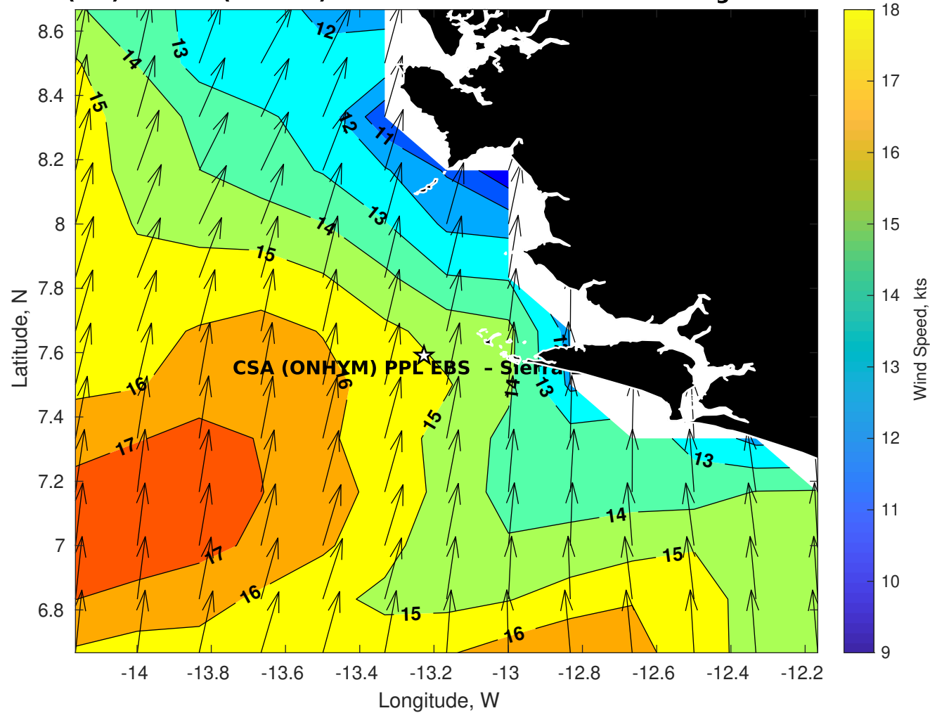
Winds (kts) for CSA (ONHYM) PPL EBS - Sierra Leone at 06-Aug-2025 09:00:00
