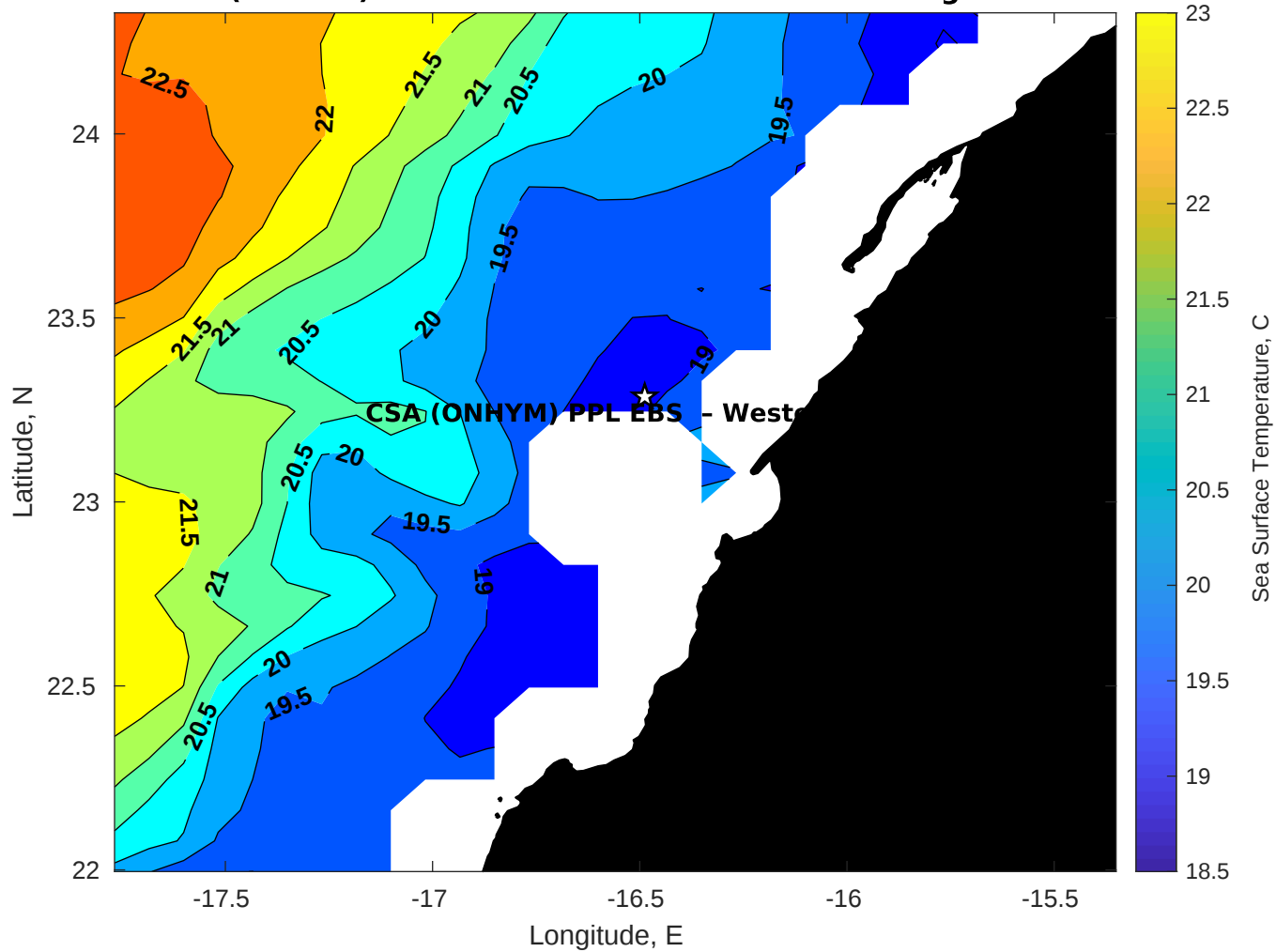
SST for CSA (ONHYM) PPL EBS - Western Sahara at 05-Aug-2025 00:00:00
