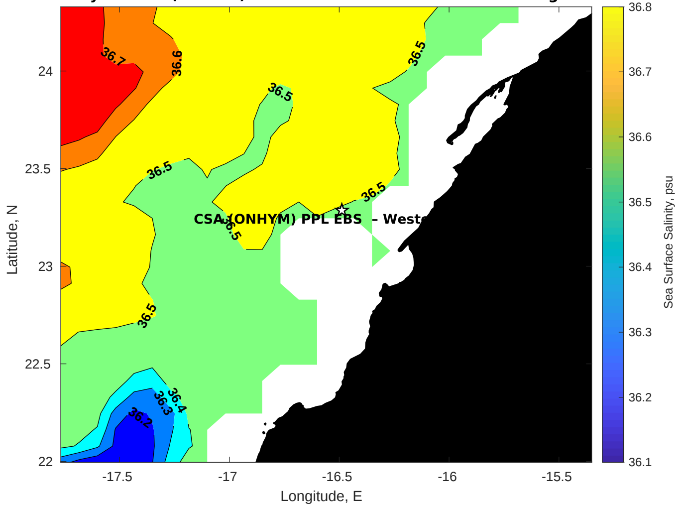
Surface Salinity for CSA (ONHYM) PPL EBS - Western Sahara at 05-Aug-2025 00:00:00
