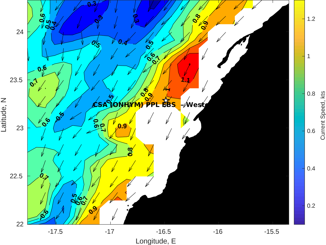
Surface Currents for CSA (ONHYM) PPL EBS - Western Sahara at 05-Aug-2025 00:00:00
