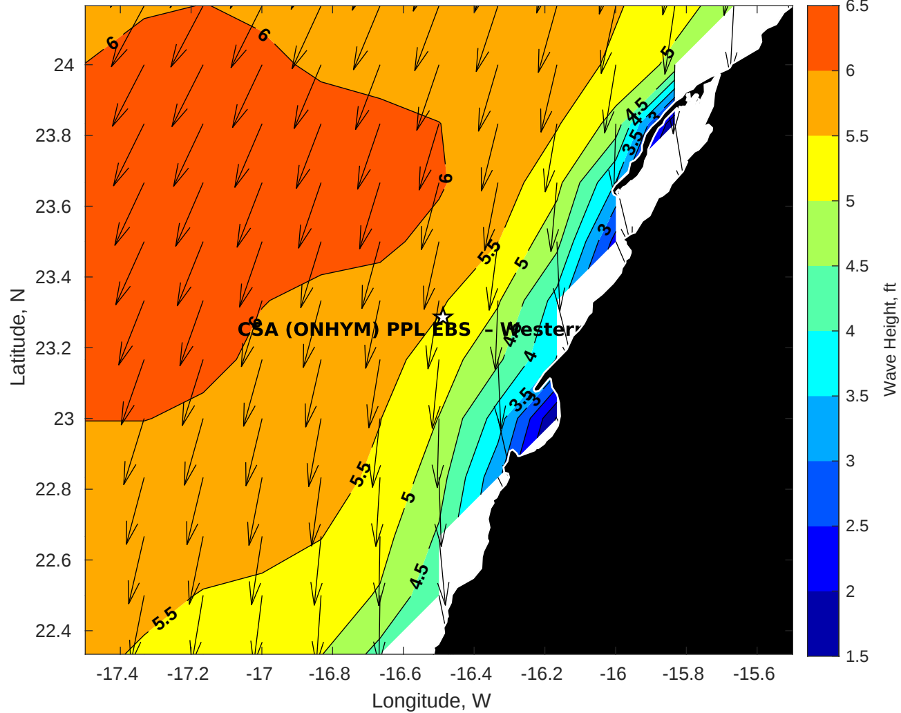
Wave Height (ft) for CSA (ONHYM) PPL EBS - Western Sahara at 06-Aug-2025 09:00:00
