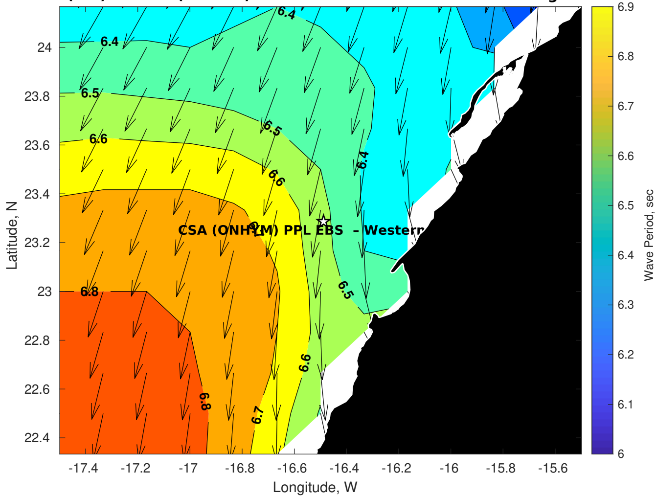
Wave Period (sec) for CSA (ONHYM) PPL EBS - Western Sahara at 06-Aug-2025 09:00:00
