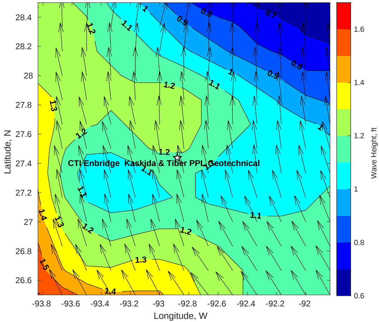
Wave Height (ft) for CTI Enbridge Kaskida & Tiber PPL Geotechnical at 06-Aug-2025 09:00:00
