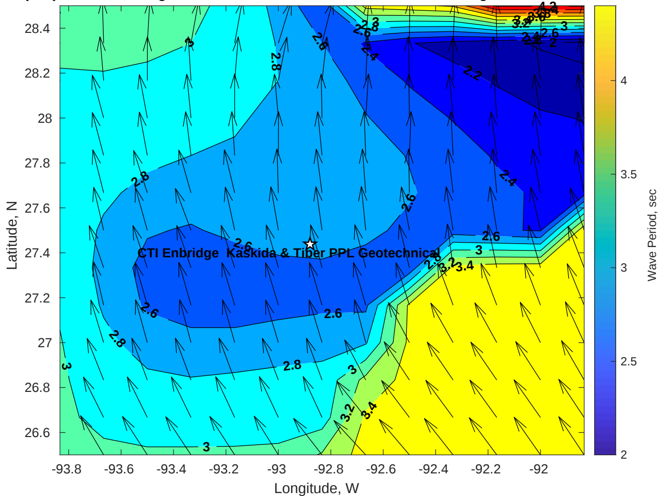
Wave Period (sec) for CTI Enbridge Kaskida & Tiber PPL Geotechnical at 06-Aug-2025 09:00:00
