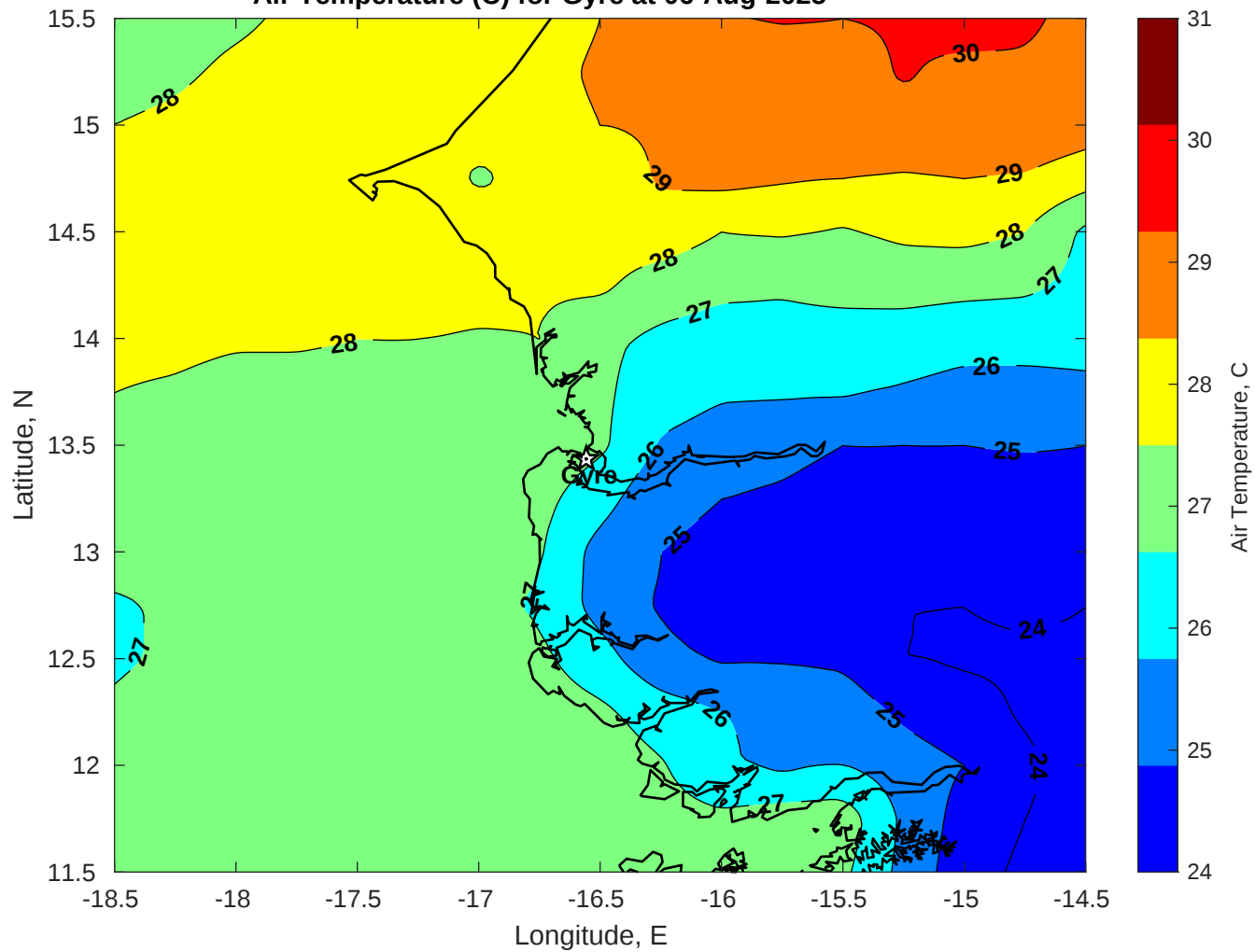
Air Temperature (C) for Gyre at 06-Aug-2025
