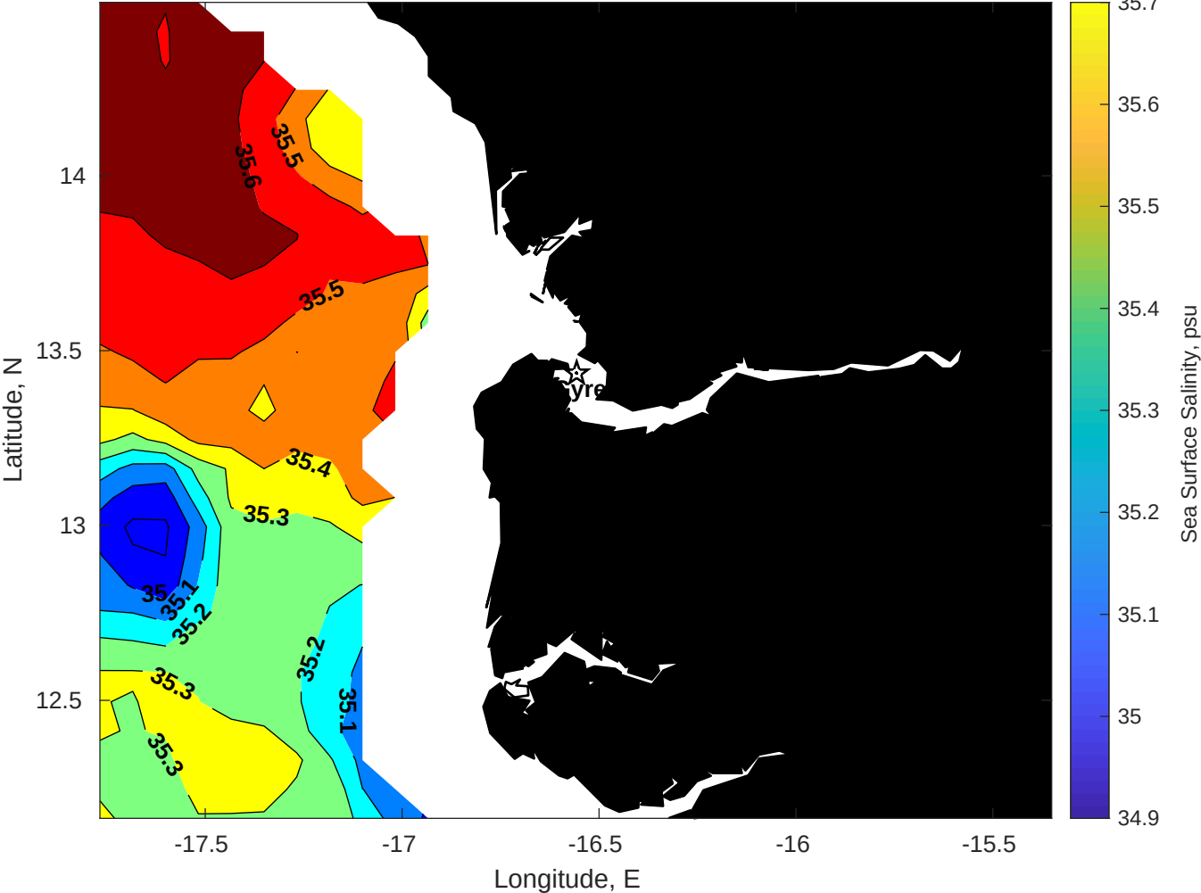
Surface Salinity for Gyre at 05-Aug-2025 00:00:00
