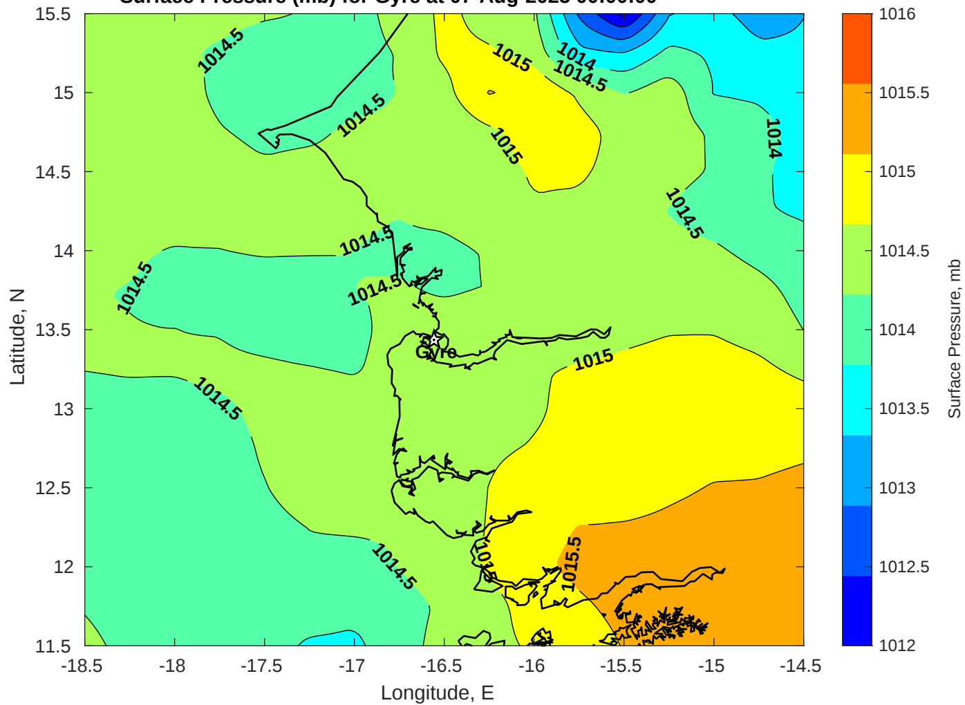
Surface Pressure (mb) for Gyre at 07-Aug-2025 00:00:00
