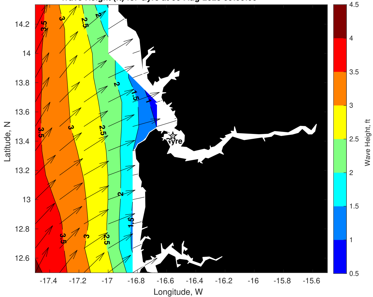
Wave Height (ft) for Gyre at 06-Aug-2025 09:00:00
