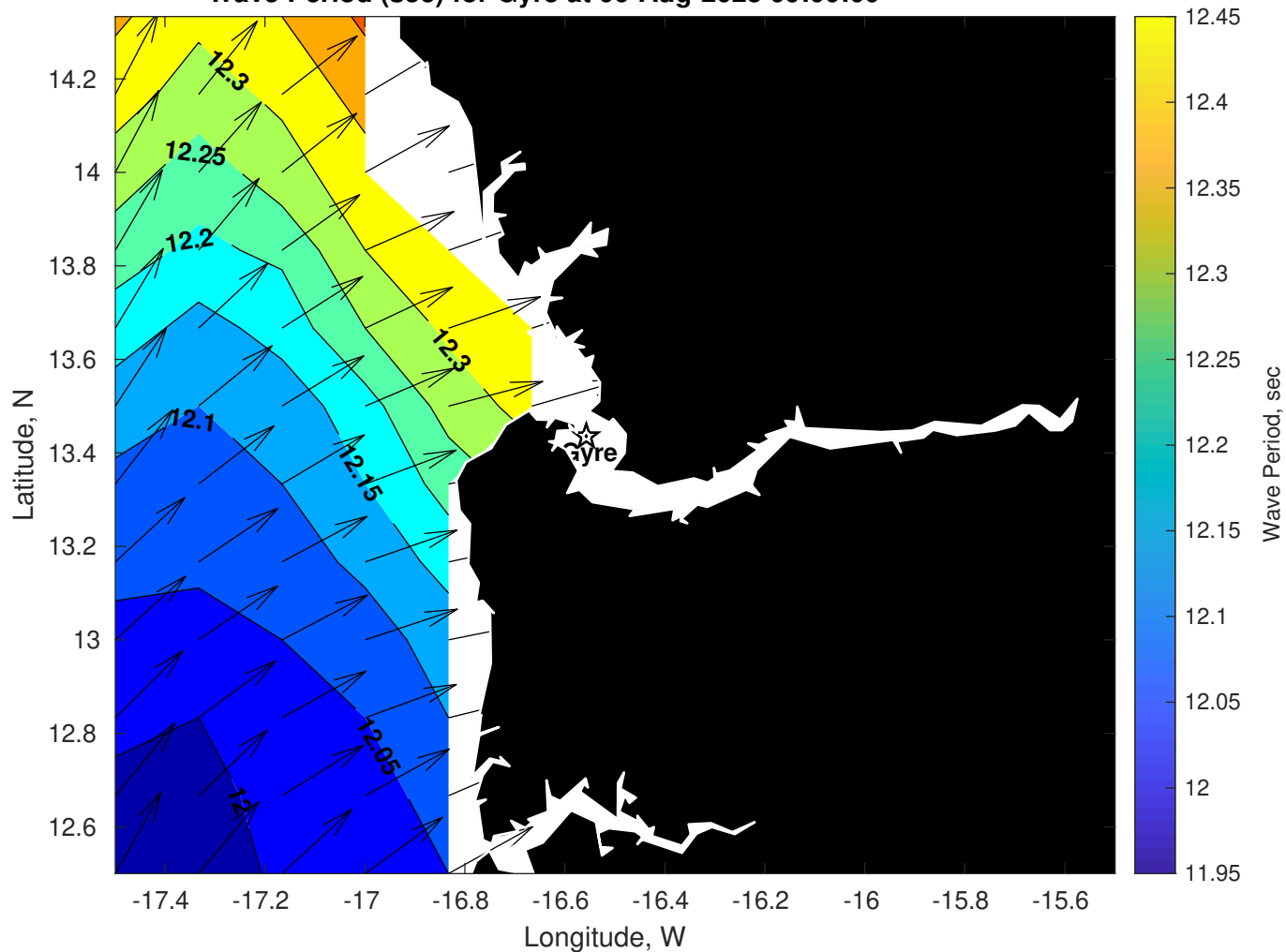
Wave Period (sec) for Gyre at 06-Aug-2025 09:00:00
