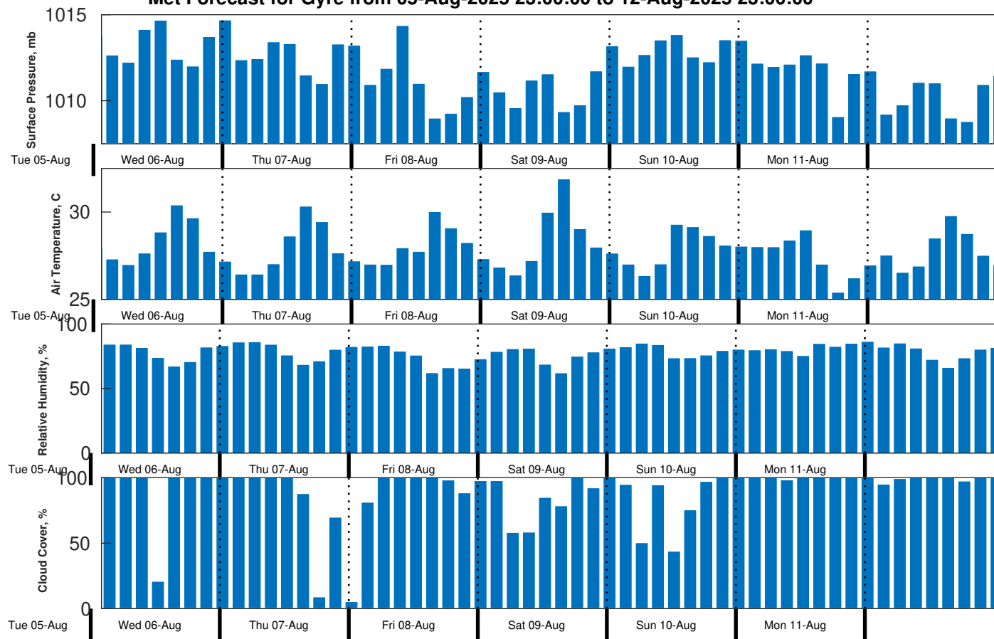
Met Forecast for Gyre from 05-Aug-2025 23:00:00 to 12-Aug-2025 23:00:00
