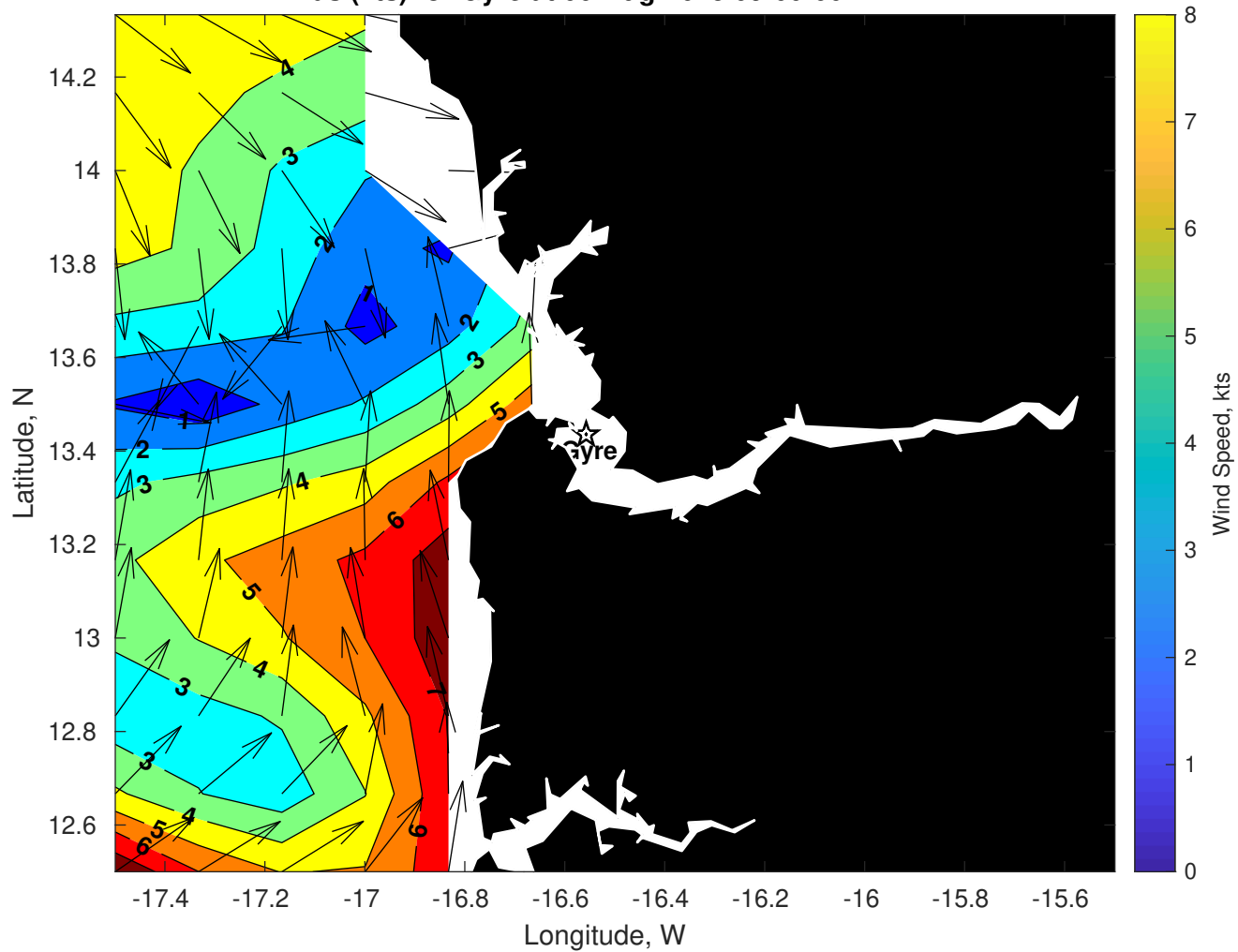
Winds (kts) for Gyre at 06-Aug-2025 09:00:00
