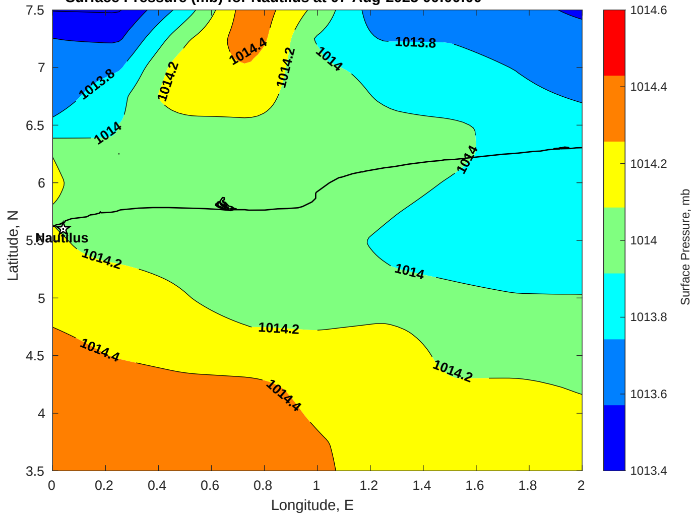
Surface Pressure (mb) for Nautilus at 07-Aug-2025 00:00:00
