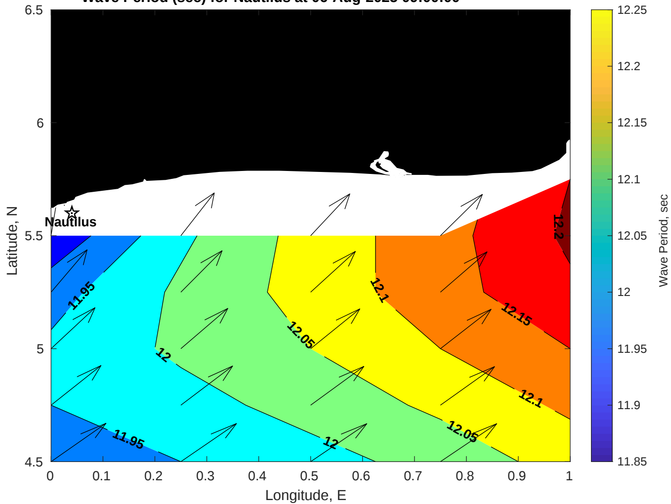
Wave Period (sec) for Nautilus at 06-Aug-2025 09:00:00
