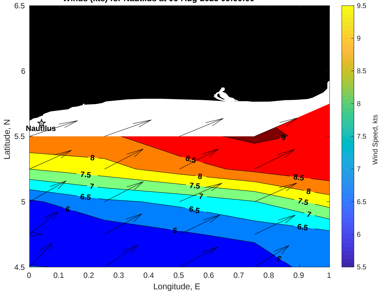
Winds (kts) for Nautilus at 06-Aug-2025 09:00:00
