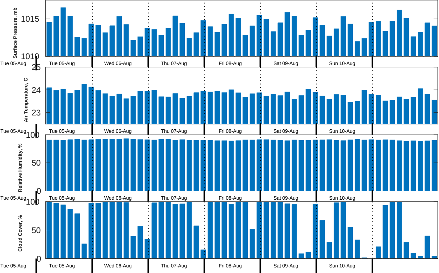
Met Forecast for Nautilus from 06-Aug-2025 00:00:00 to 13-Aug-2025 00:00:00
