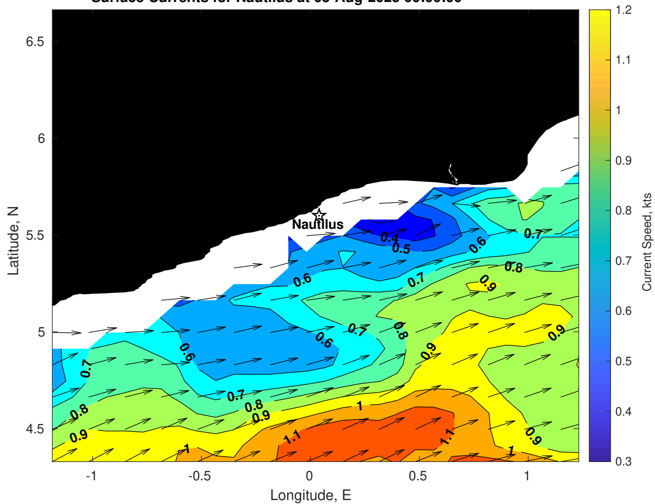
Surface Currents for Nautilus at 05-Aug-2025 00:00:00
