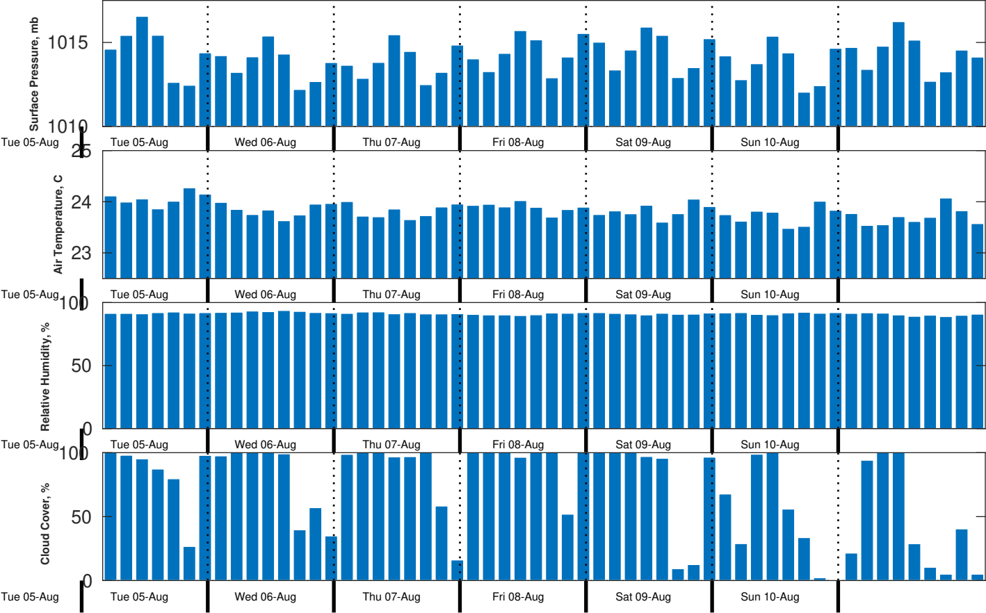
Met Forecast for Nautilus from 06-Aug-2025 00:00:00 to 13-Aug-2025 00:00:00
