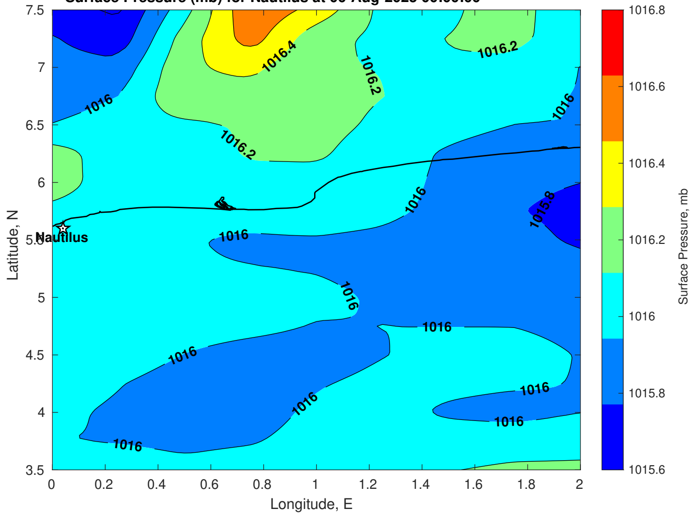
Surface Pressure (mb) for Nautilus at 06-Aug-2025 00:00:00
