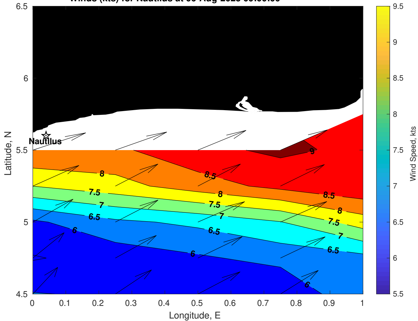
Winds (kts) for Nautilus at 06-Aug-2025 09:00:00
