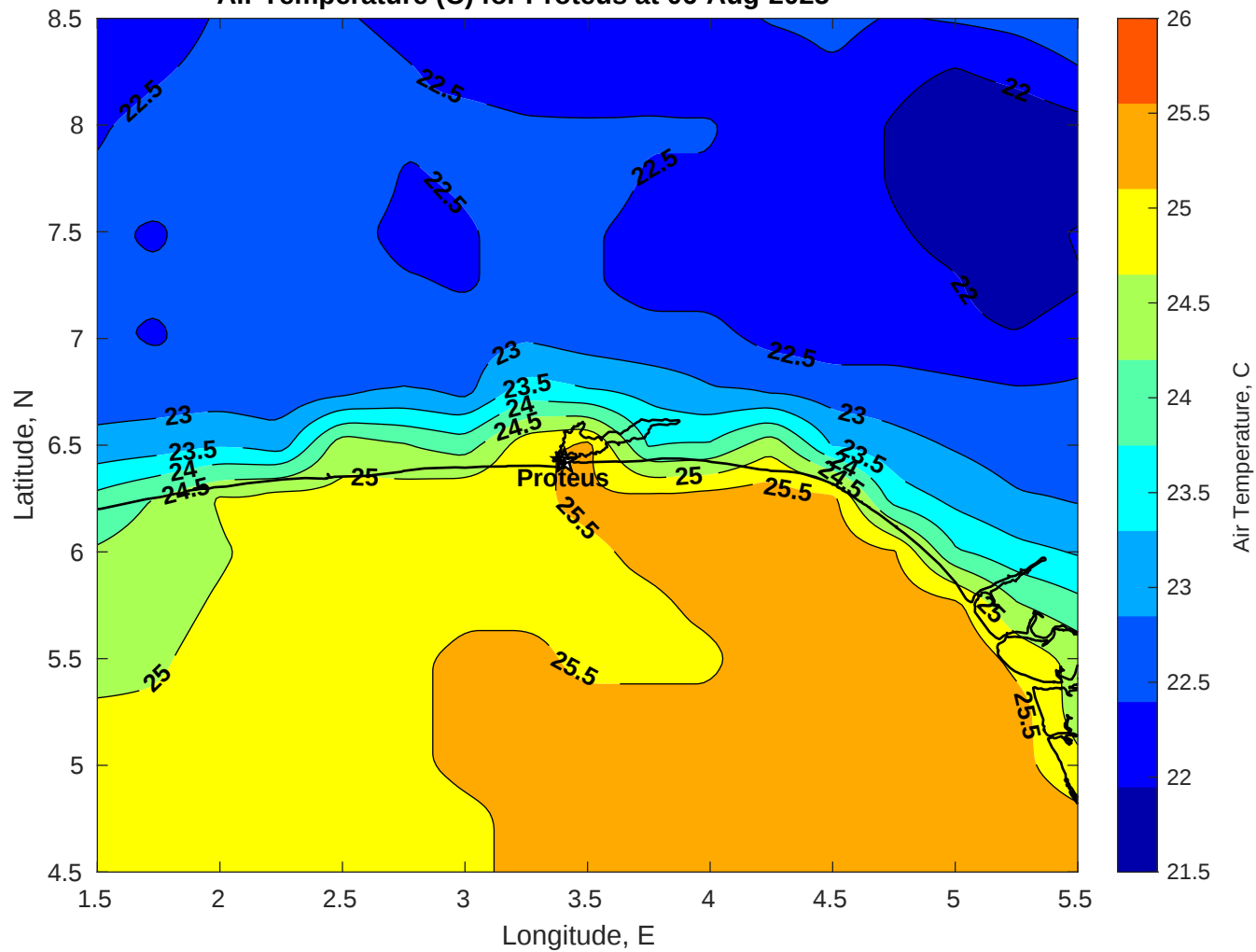
Air Temperature (C) for Proteus at 06-Aug-2025
