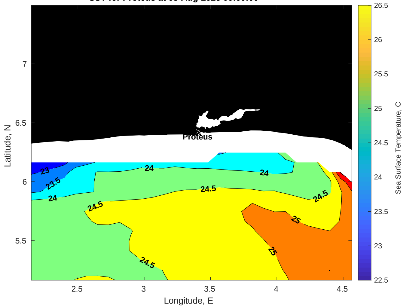
SST for Proteus at 05-Aug-2025 00:00:00
