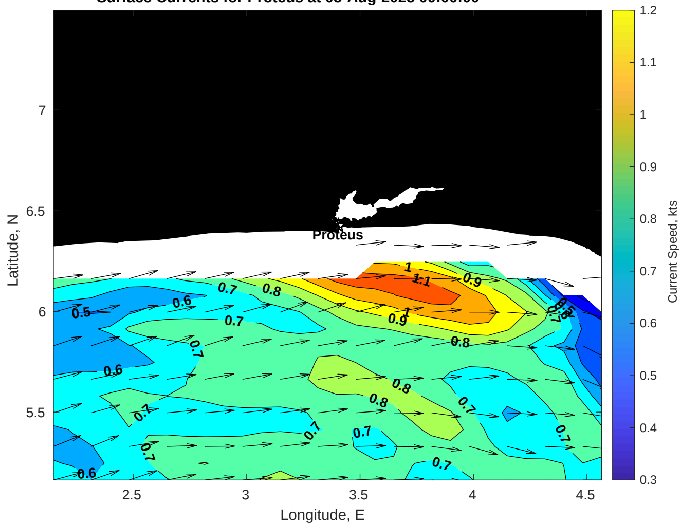
Surface Currents for Proteus at 05-Aug-2025 00:00:00
