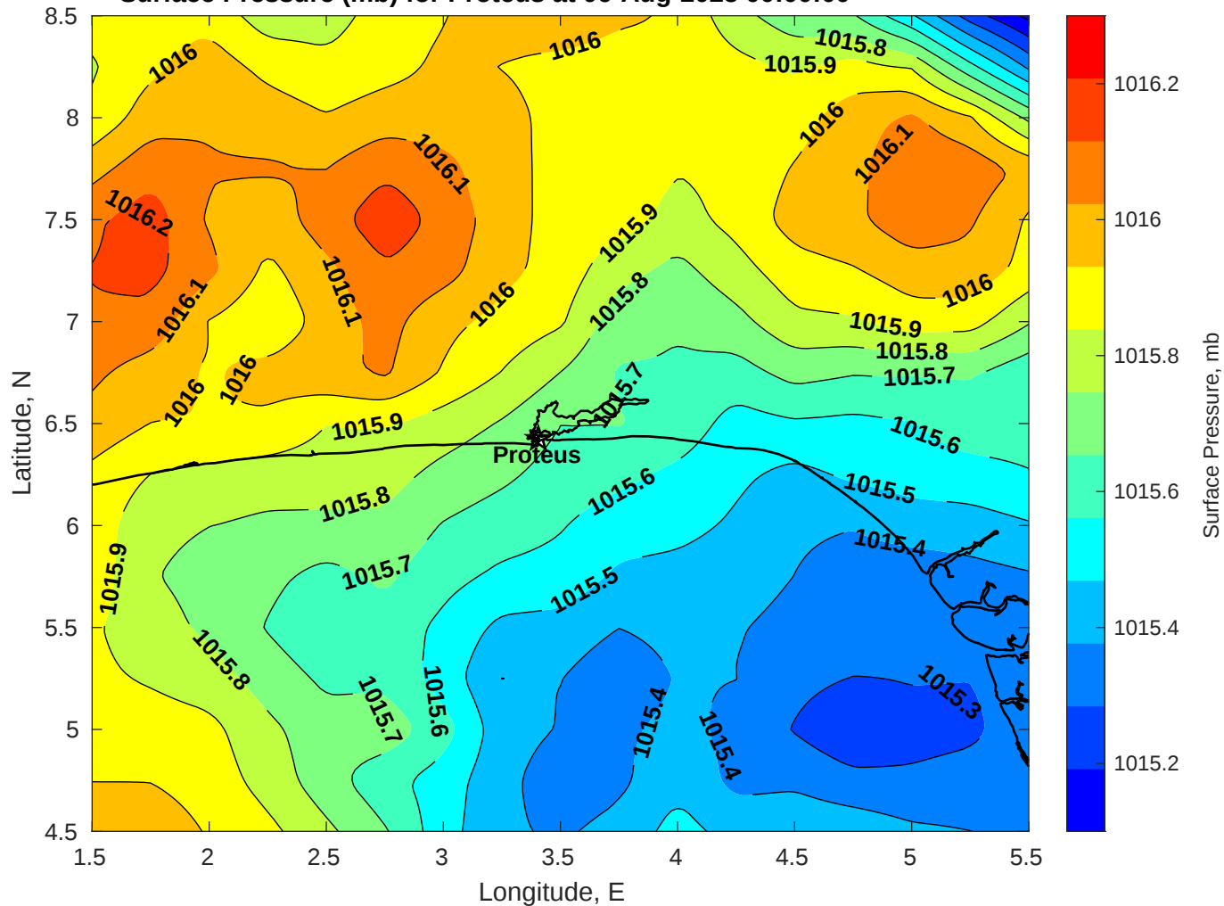
Surface Pressure (mb) for Proteus at 06-Aug-2025 00:00:00
