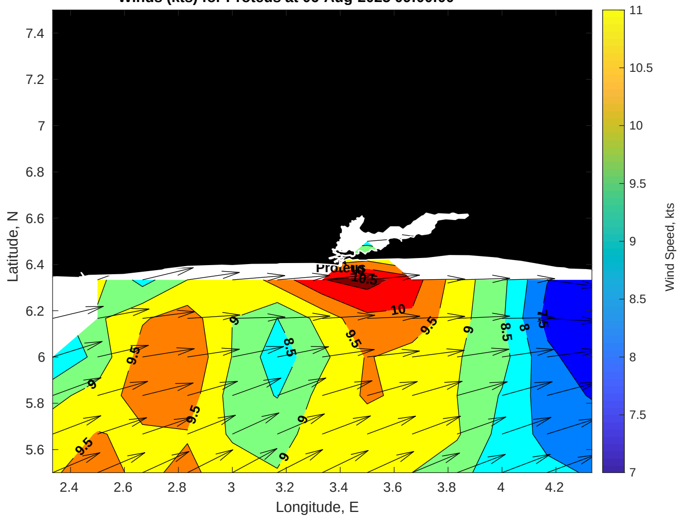
Winds (kts) for Proteus at 06-Aug-2025 09:00:00
