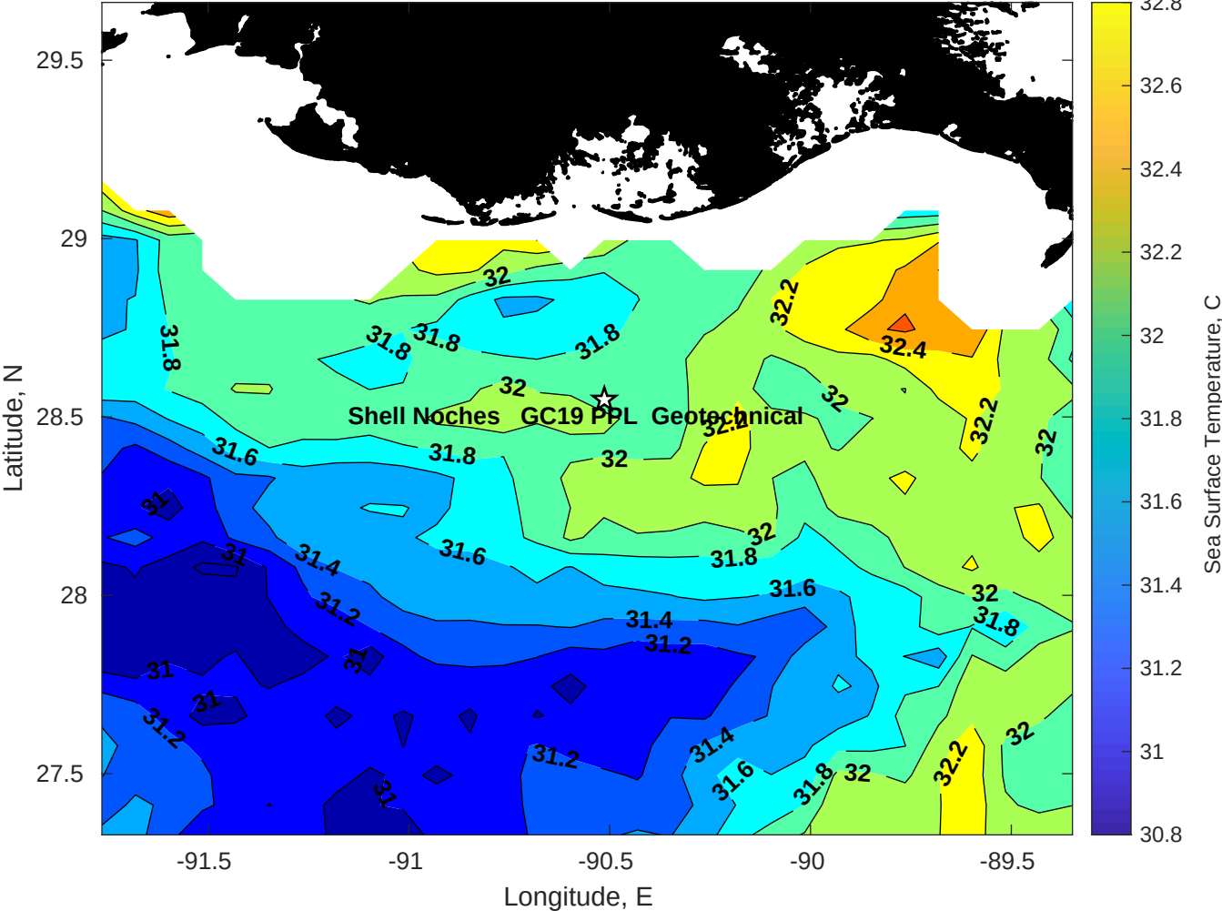
SST for Shell Noches GC19 PPL Geotechnical at 05-Aug-2025 00:00:00
