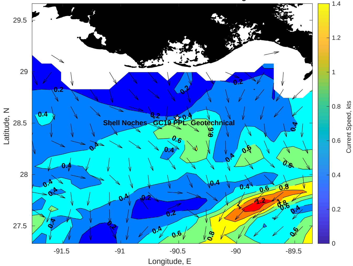
Surface Currents for Shell Noches GC19 PPL Geotechnical at 05-Aug-2025 00:00:00
