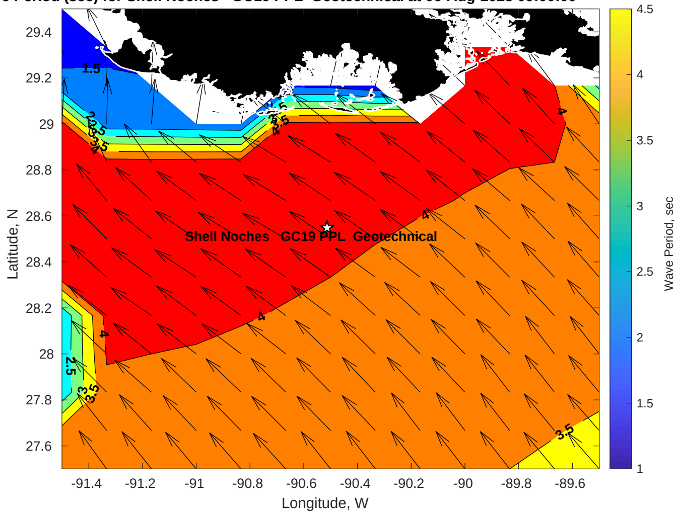
Wave Period (sec) for Shell Noches GC19 PPL Geotechnical at 06-Aug-2025 09:00:00
