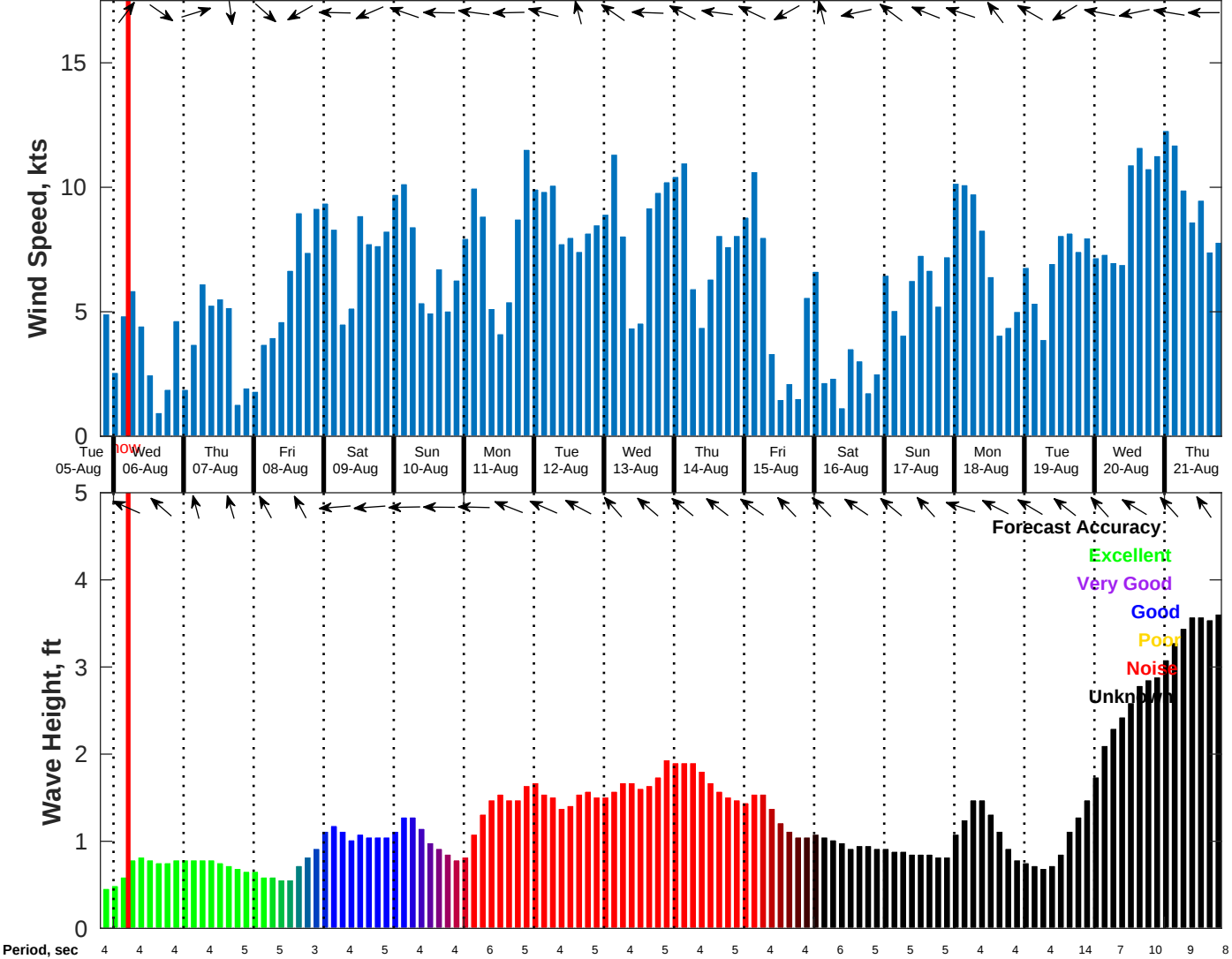
Wind & Wave Forecast for Shell Noches GC19 PPL Geotechnical from 05-Aug-2025 20:00:00 to 21-Aug-2025 20:00:00
