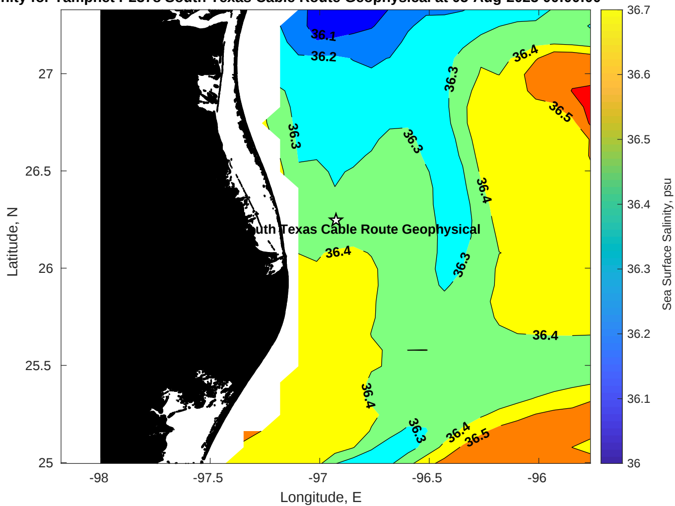
Surface Salinity for Tampnet P2378 South Texas Cable Route Geophysical at 05-Aug-2025 00:00:00
