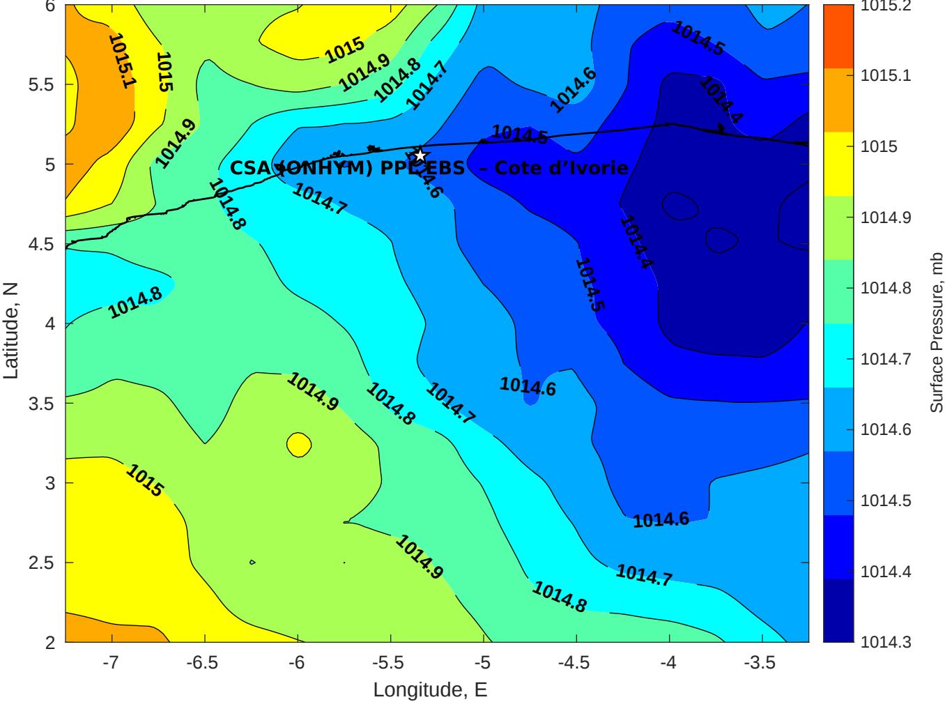
Surface Pressure (mb) for CSA (ONHYM) PPL EBS - Cote d'Ivoire at 09-Aug-2025 00:00:00
