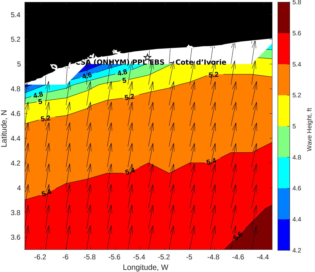
Wave Height (ft) for CSA (ONHYM) PPL EBS - Cote d'Ivoire at 07-Aug-2025 09:00:00
