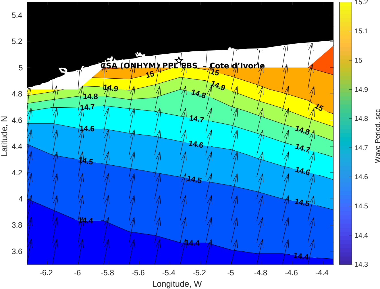
Wave Period (sec) for CSA (ONHYM) PPL EBS - Cote d'Ivoire at 07-Aug-2025 09:00:00
