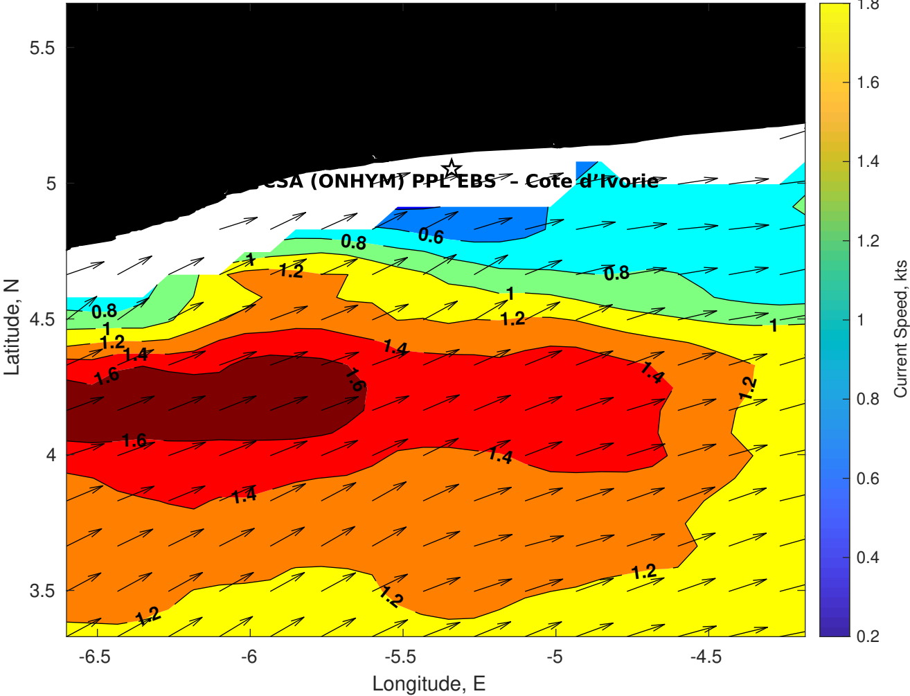
Surface Currents for CSA (ONHYM) PPL EBS - Cote d'Ivoire at 06-Aug-2025 00:00:00
