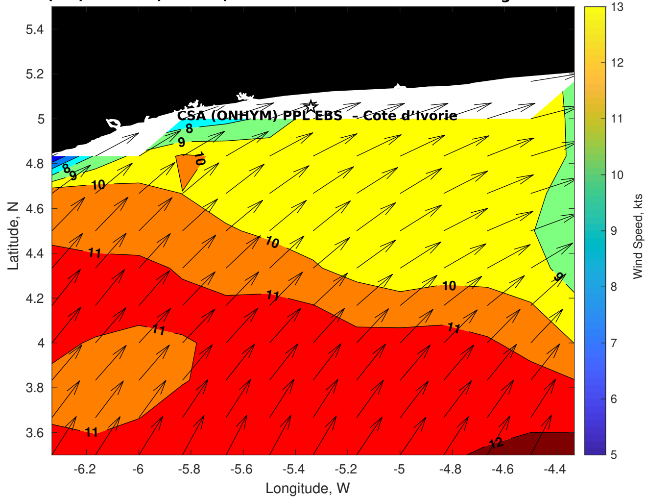
Winds (kts) for CSA (ONHYM) PPL EBS - Cote d'Ivoire at 07-Aug-2025 09:00:00
