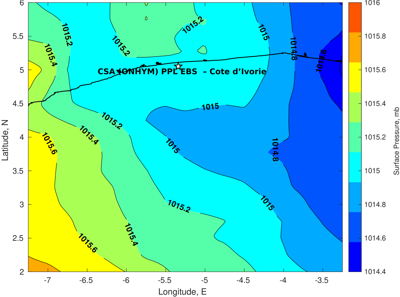
Surface Pressure (mb) for CSA (ONHYM) PPL EBS - Cote d'Ivoire at 07-Aug-2025 00:00:00
