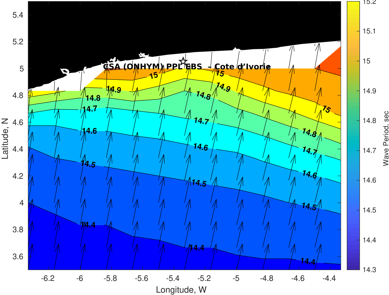
Wave Period (sec) for CSA (ONHYM) PPL EBS - Cote d'Ivoire at 07-Aug-2025 09:00:00
