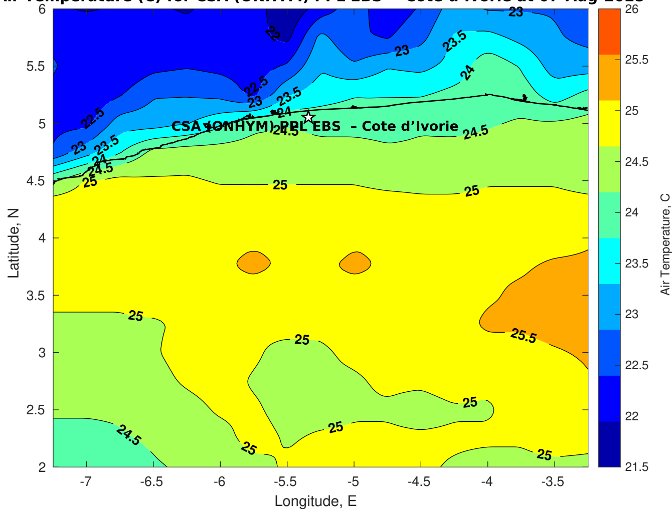
Air Temperature (C) for CSA (ONHYM) PPL EBS - Cote d'Ivoire at 07-Aug-2025
