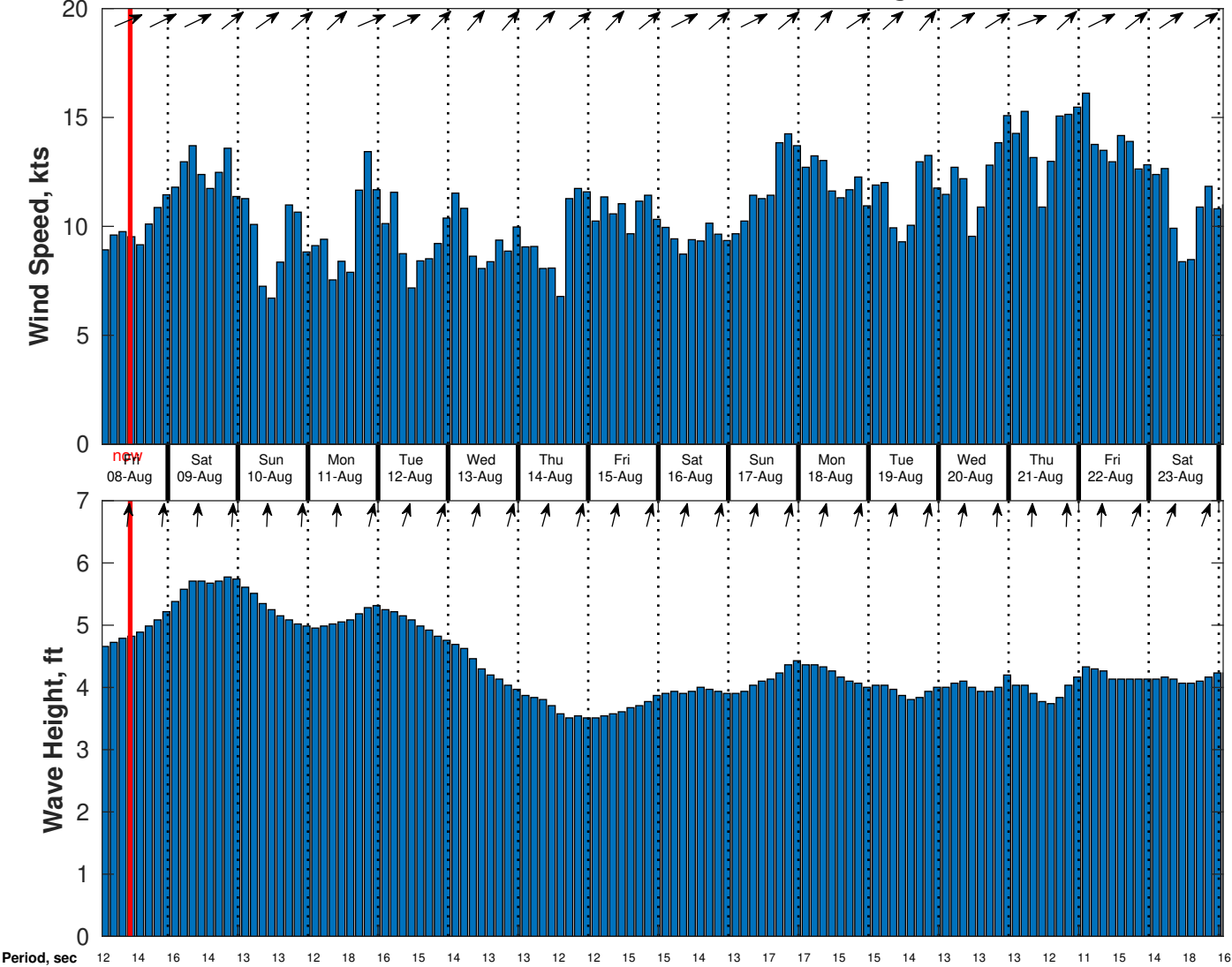
Wind & Wave Forecast for CSA (ONHYM) PPL EBS - Cote d'Ivoire from 07-Aug-2025 01:00:00 to 23-Aug-2025 01:00:00
