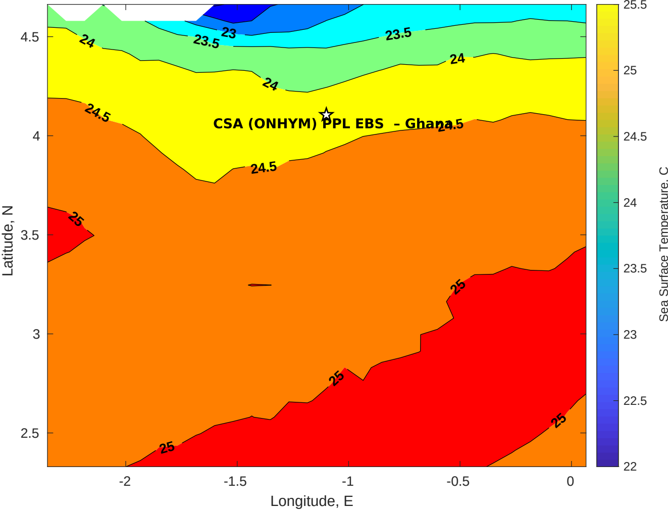
SST for CSA (ONHYM) PPL EBS - Ghana at 06-Aug-2025 00:00:00
