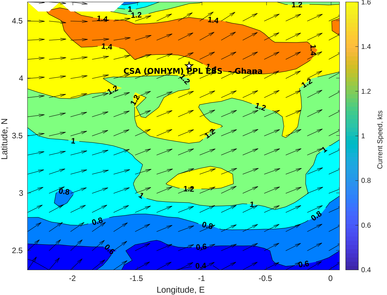
Surface Currents for CSA (ONHYM) PPL EBS - Ghana at 06-Aug-2025 00:00:00
