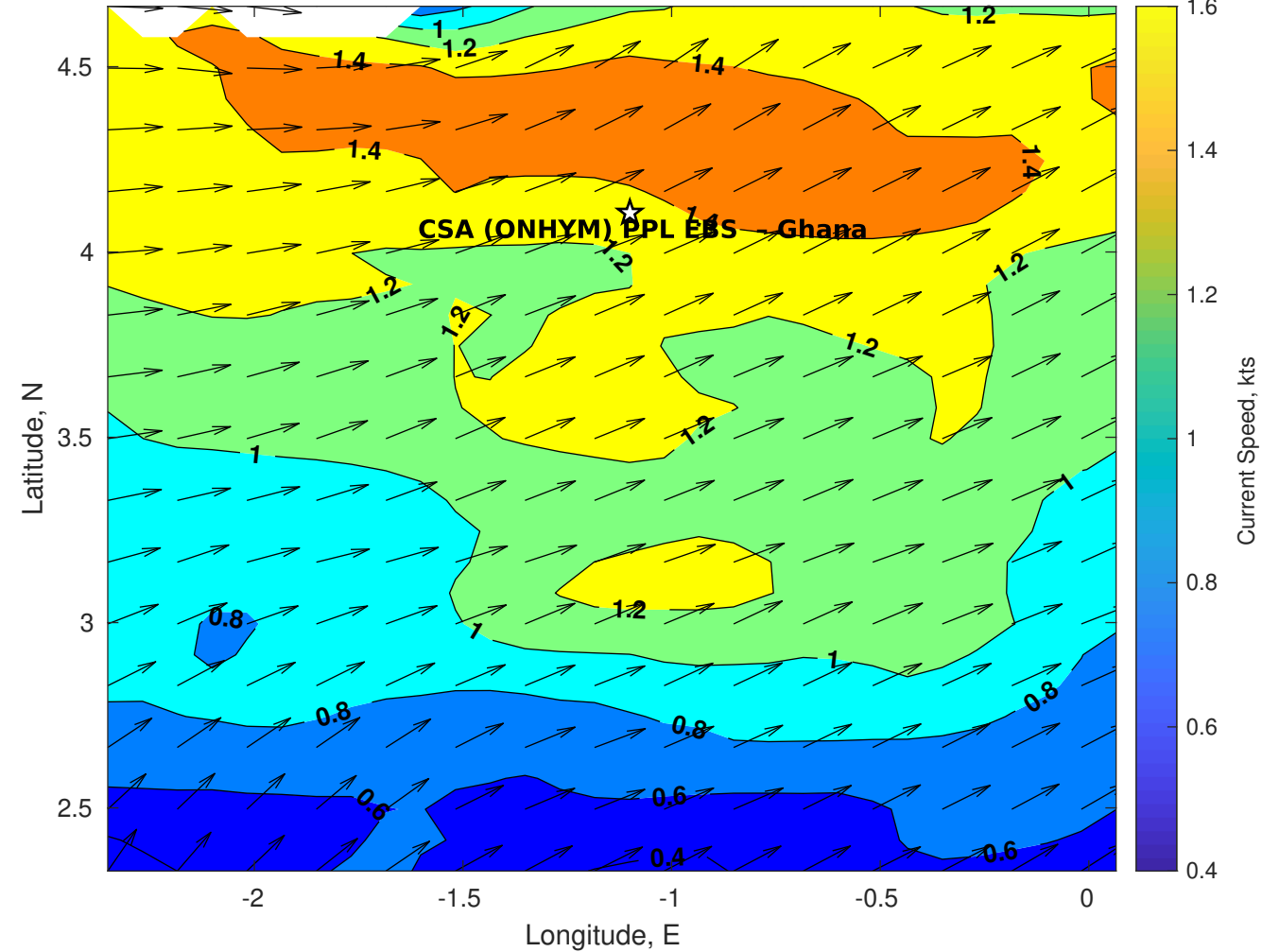
Surface Currents for CSA (ONHYM) PPL EBS - Ghana at 06-Aug-2025 00:00:00
