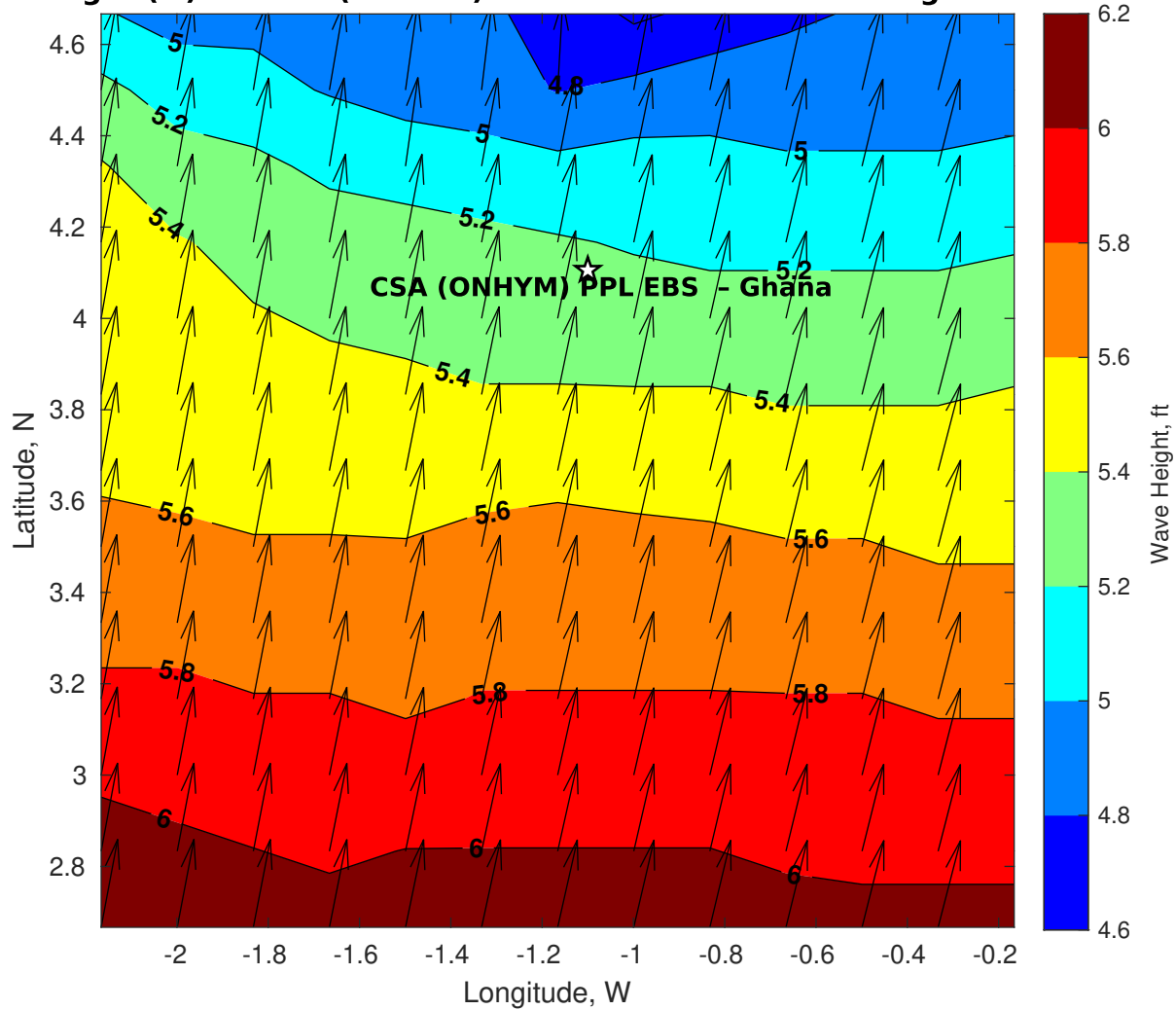
Wave Height (ft) for CSA (ONHYM) PPL EBS - Ghana at 07-Aug-2025 09:00:00
