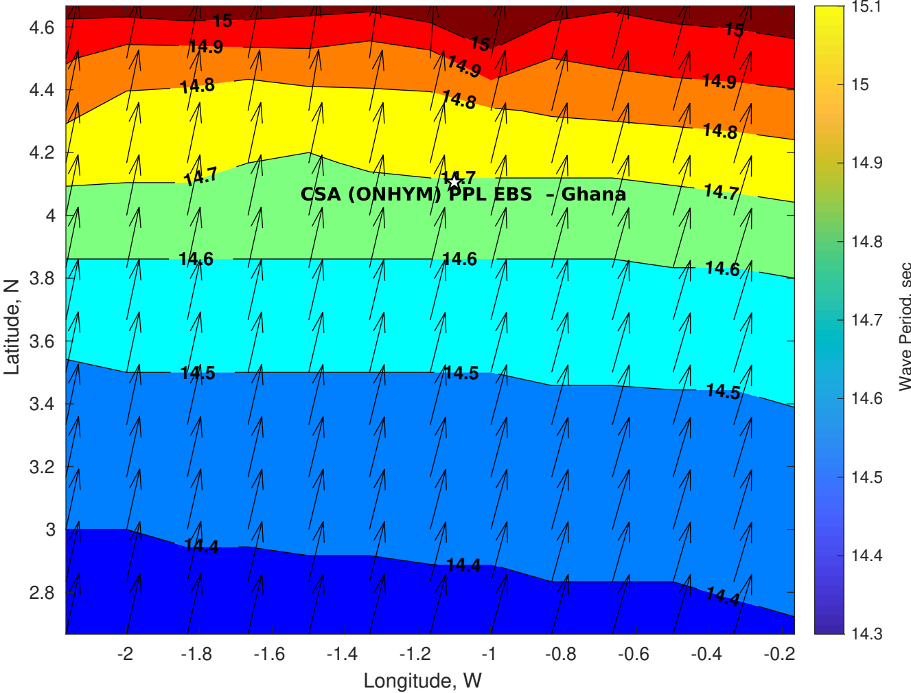
Wave Period (sec) for CSA (ONHYM) PPL EBS - Ghana at 07-Aug-2025 09:00:00
