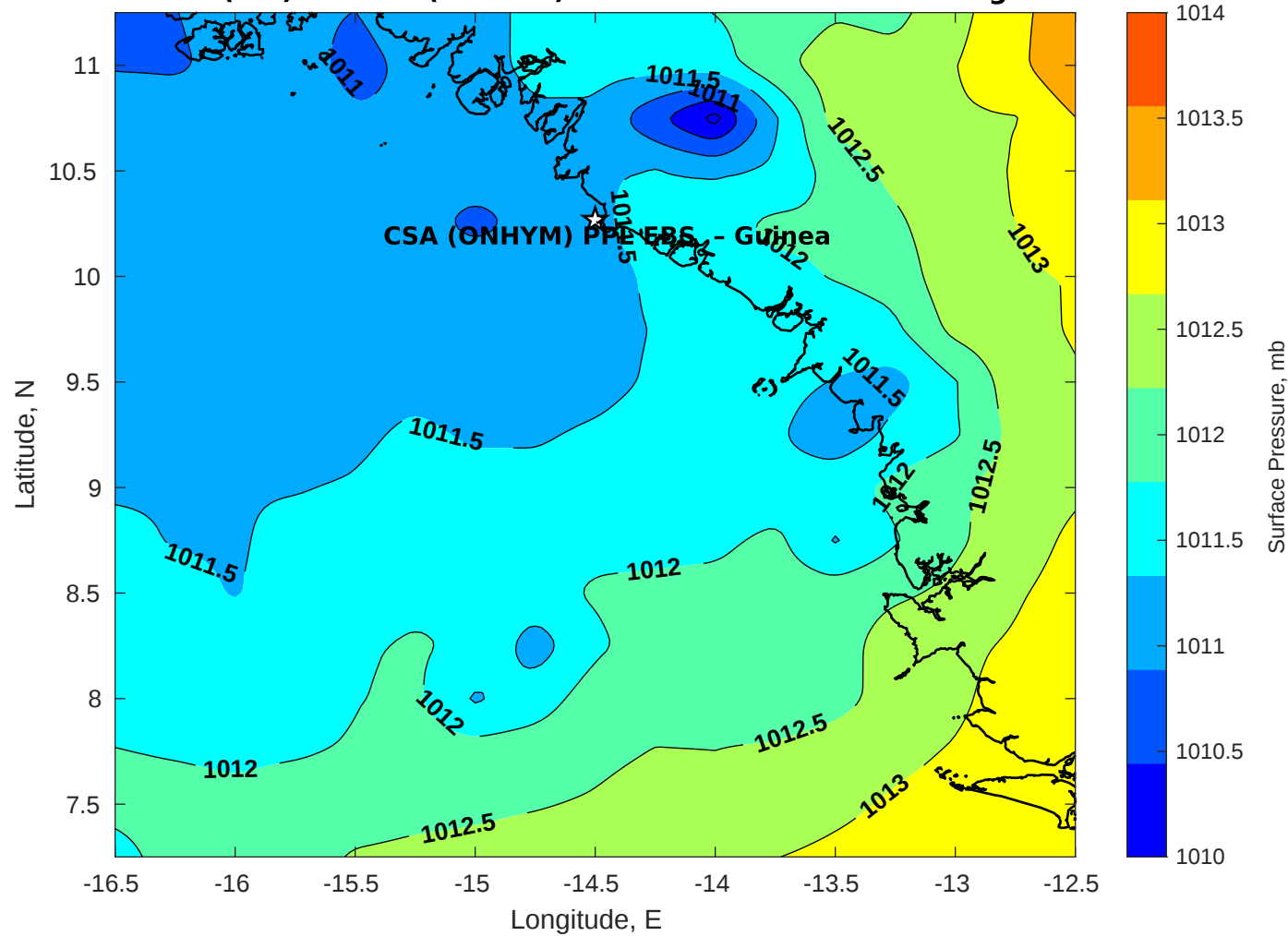
Surface Pressure (mb) for CSA (ONHYM) PPL EBS - Guinea at 09-Aug-2025 00:00:00
