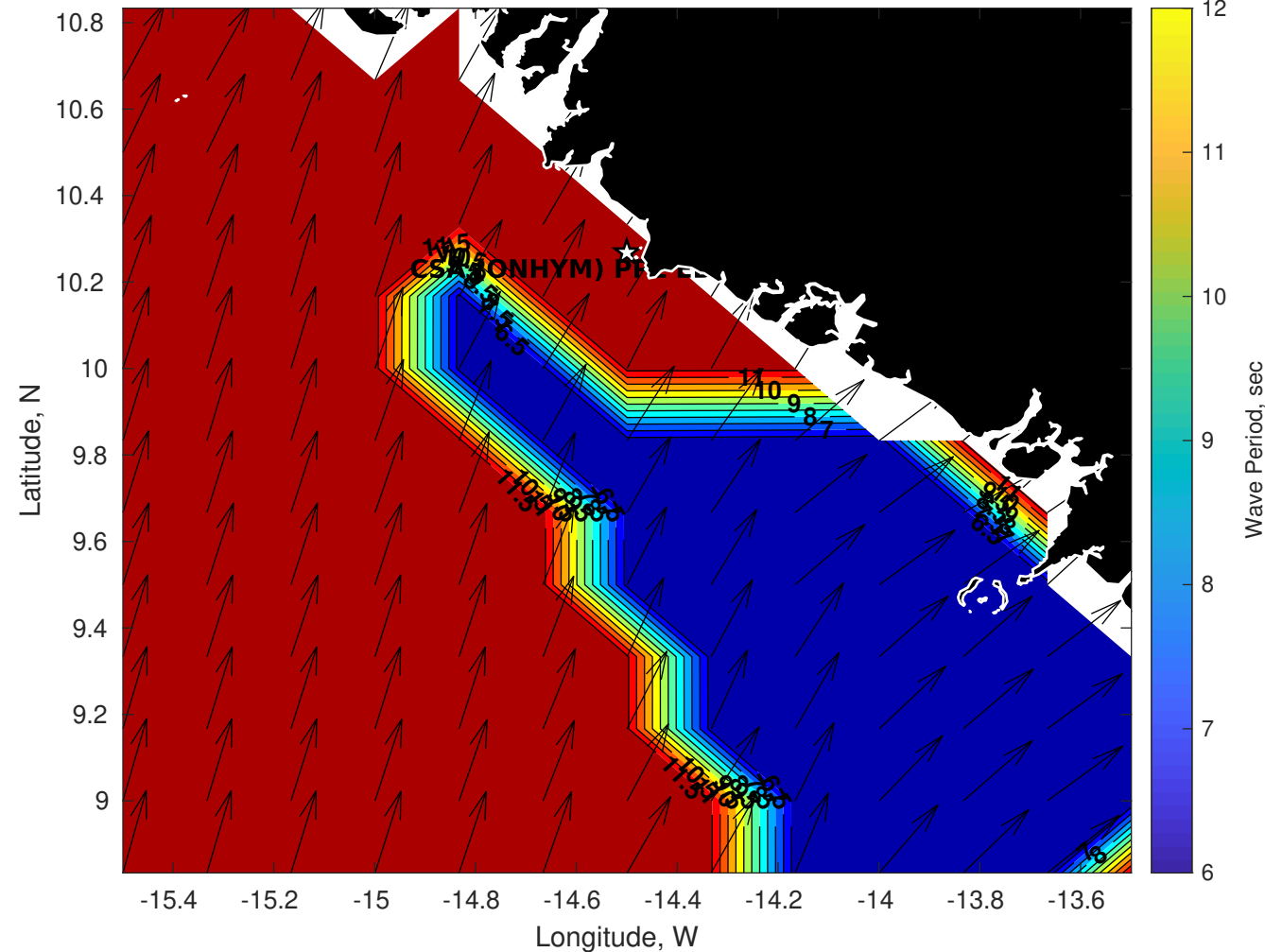
Wave Period (sec) for CSA (ONHYM) PPL EBS - Guinea at 07-Aug-2025 09:00:00
