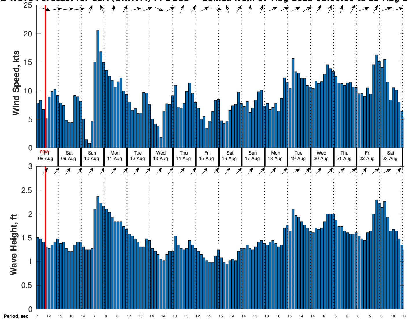
Wind & Wave Forecast for CSA (ONHYM) PPL EBS - Guinea from 07-Aug-2025 01:00:00 to 23-Aug-2025 01:00:00
