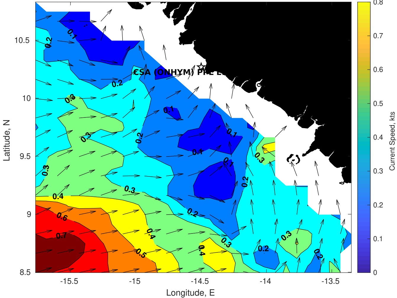
Surface Currents for CSA (ONHYM) PPL EBS - Guinea at 06-Aug-2025 00:00:00
