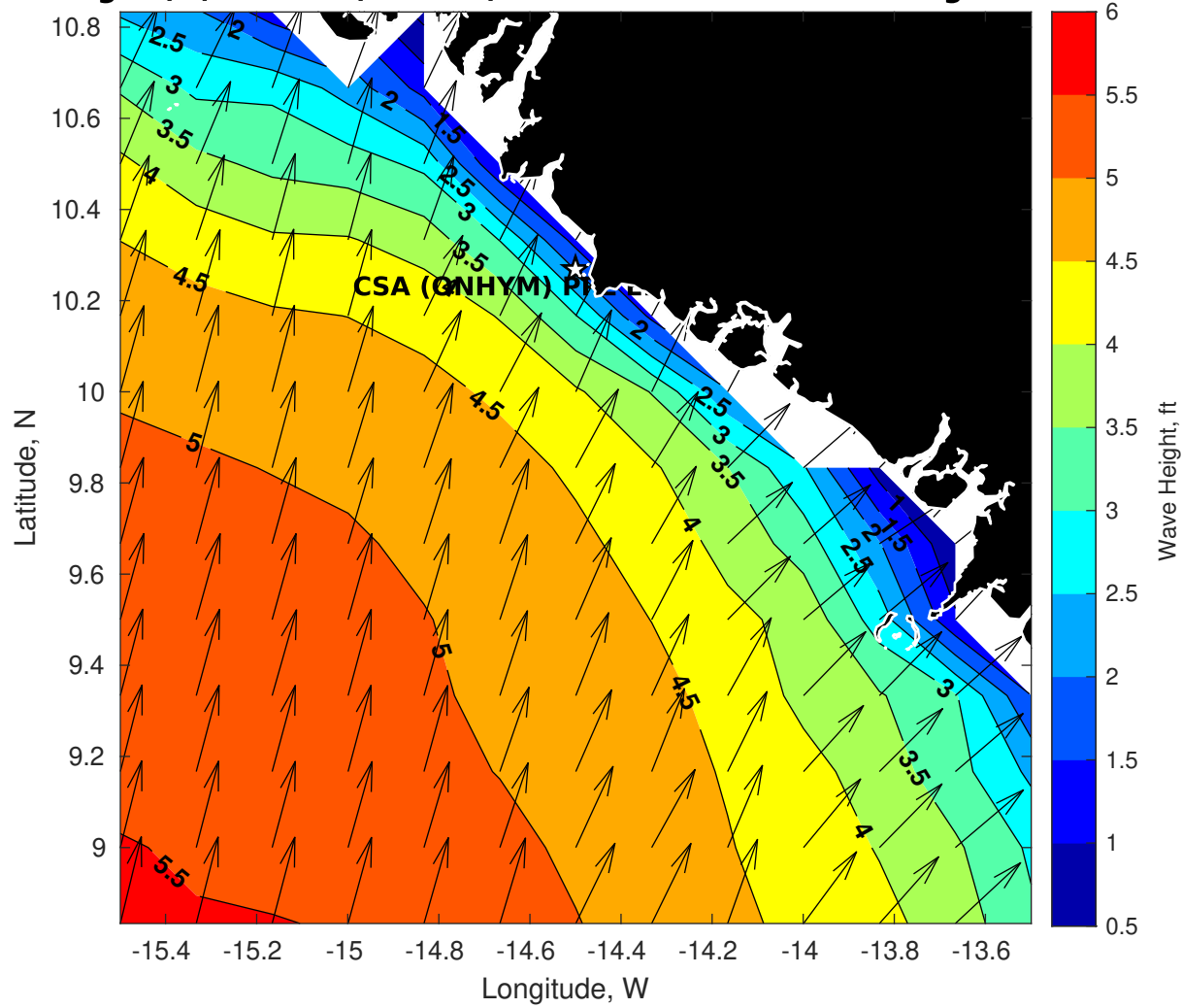
Wave Height (ft) for CSA (ONHYM) PPL EBS - Guinea at 07-Aug-2025 09:00:00
