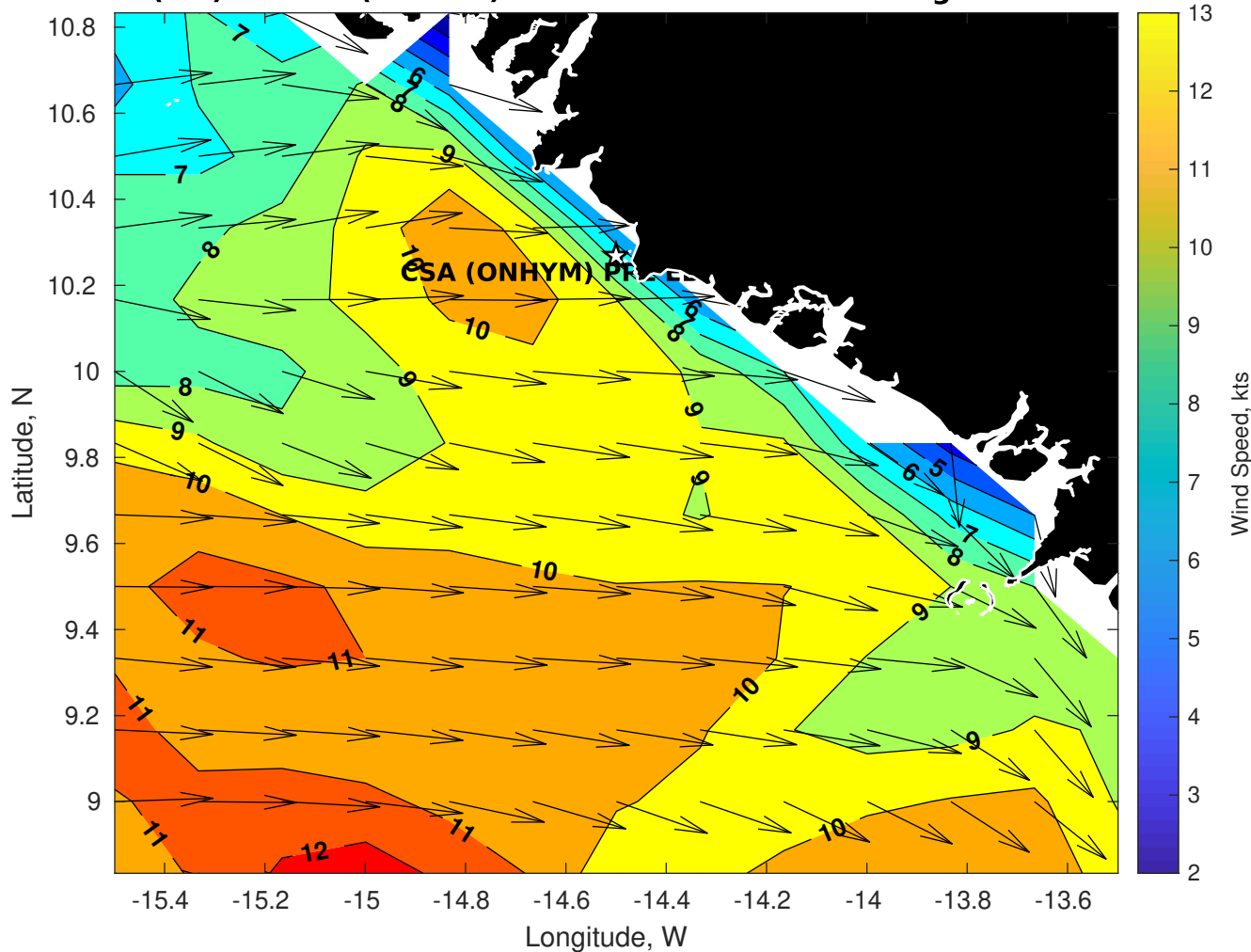
Winds (kts) for CSA (ONHYM) PPL EBS - Guinea at 07-Aug-2025 09:00:00
