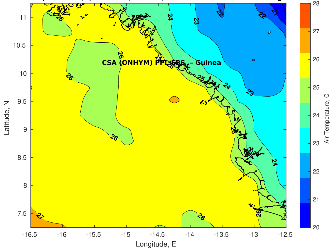
Air Temperature (C) for CSA (ONHYM) PPL EBS - Guinea at 07-Aug-2025
