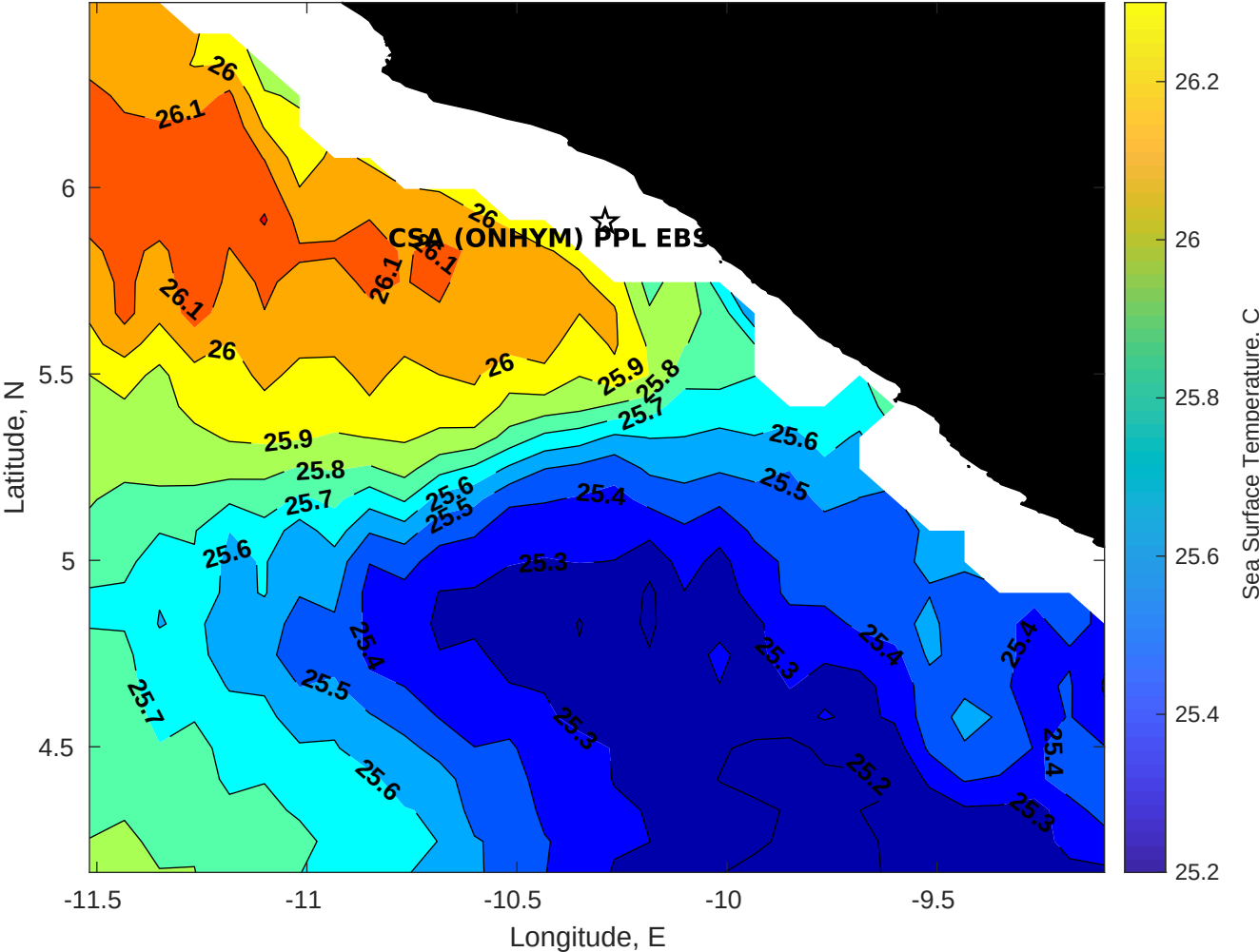
SST for CSA (ONHYM) PPL EBS - Liberia at 06-Aug-2025 00:00:00
