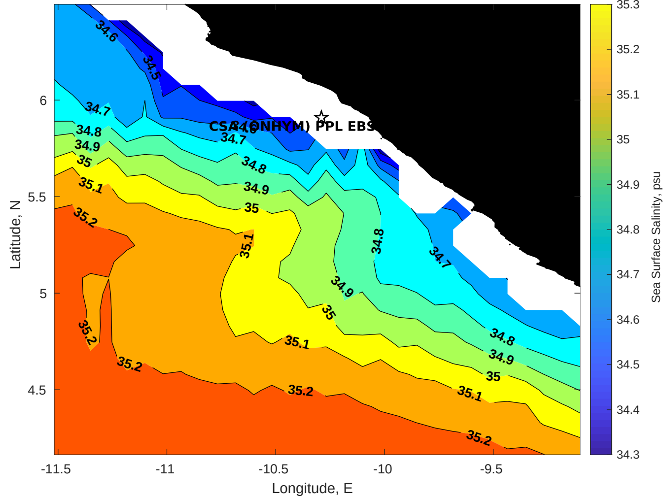
Surface Salinity for CSA (ONHYM) PPL EBS - Liberia at 06-Aug-2025 00:00:00
