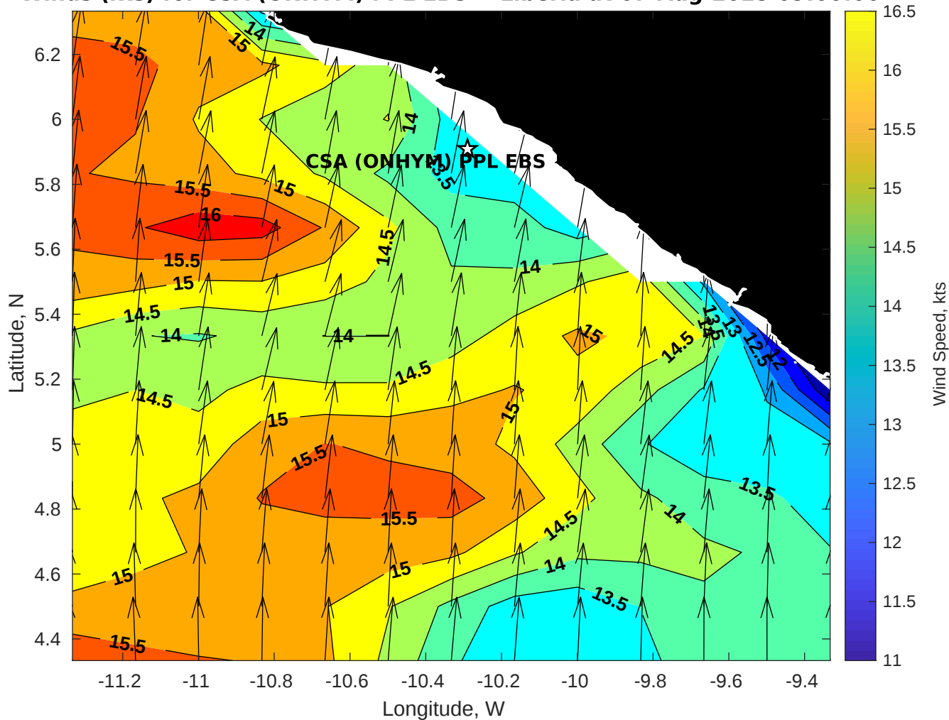
Winds (kts) for CSA (ONHYM) PPL EBS - Liberia at 07-Aug-2025 09:00:00
