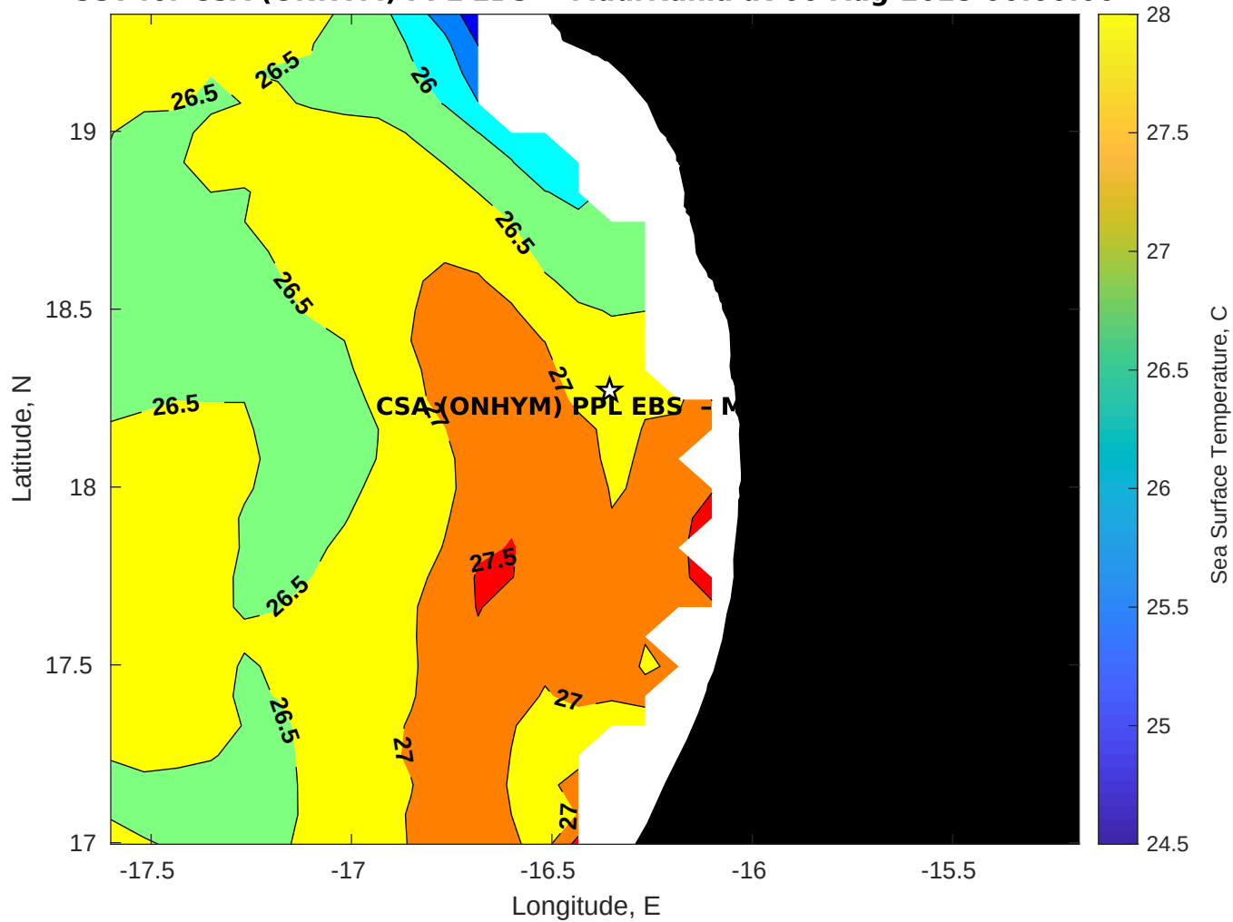
SST for CSA (ONHYM) PPL EBS - Mauritania at 06-Aug-2025 00:00:00
