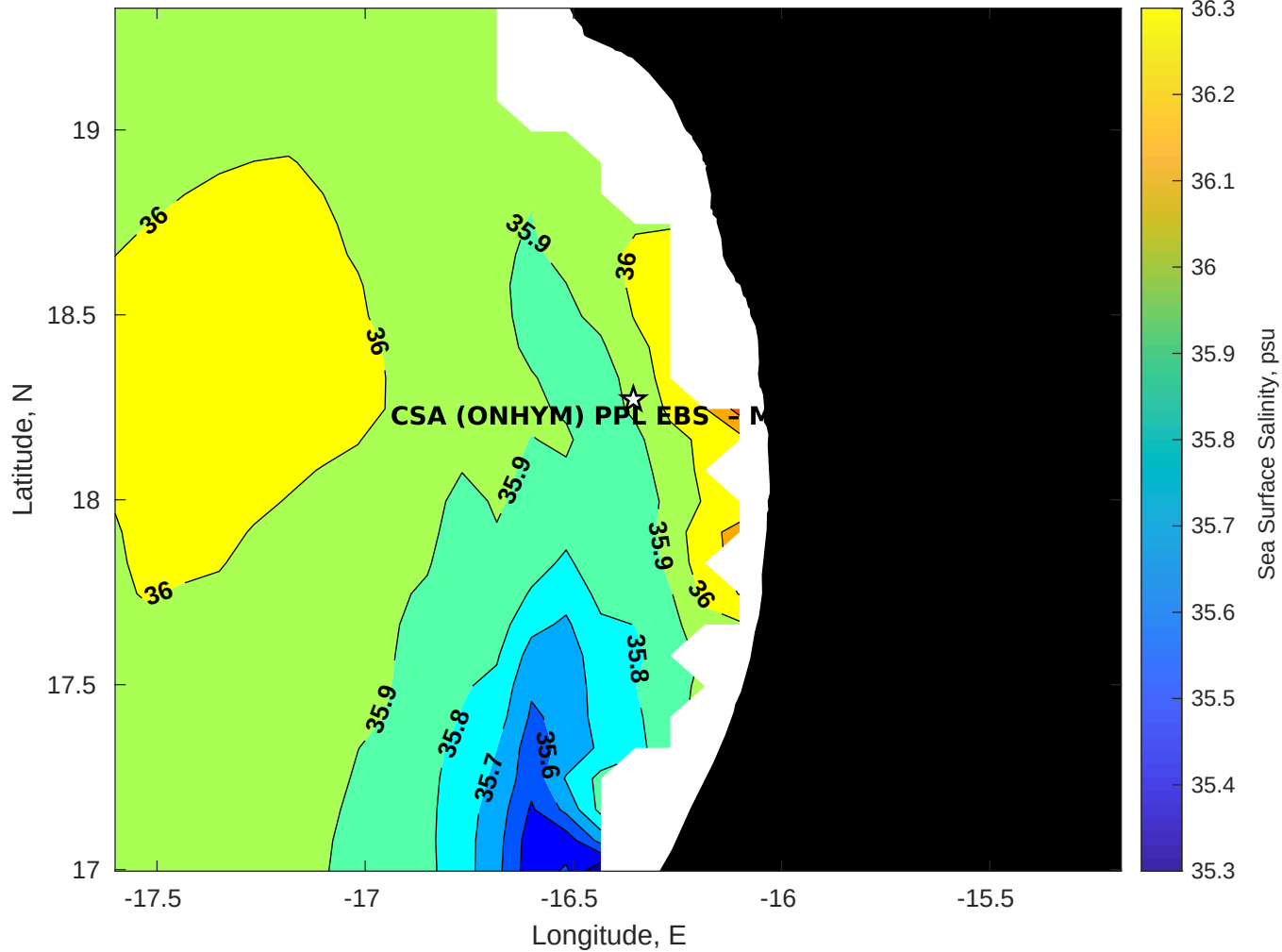
Surface Salinity for CSA (ONHYM) PPL EBS - Mauritania at 06-Aug-2025 00:00:00
