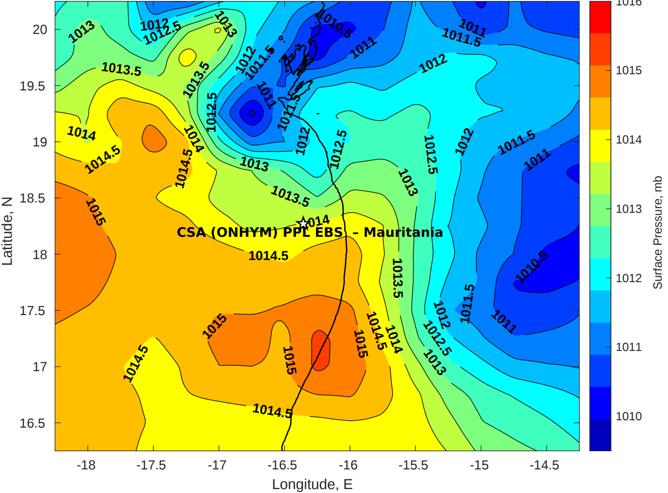
Surface Pressure (mb) for CSA (ONHYM) PPL EBS - Mauritania at 07-Aug-2025 00:00:00
