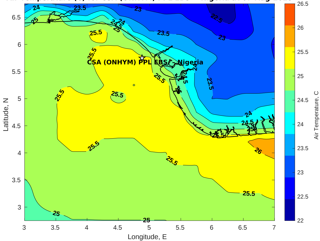
Air Temperature (C) for CSA (ONHYM) PPL EBS - Nigeria at 07-Aug-2025
