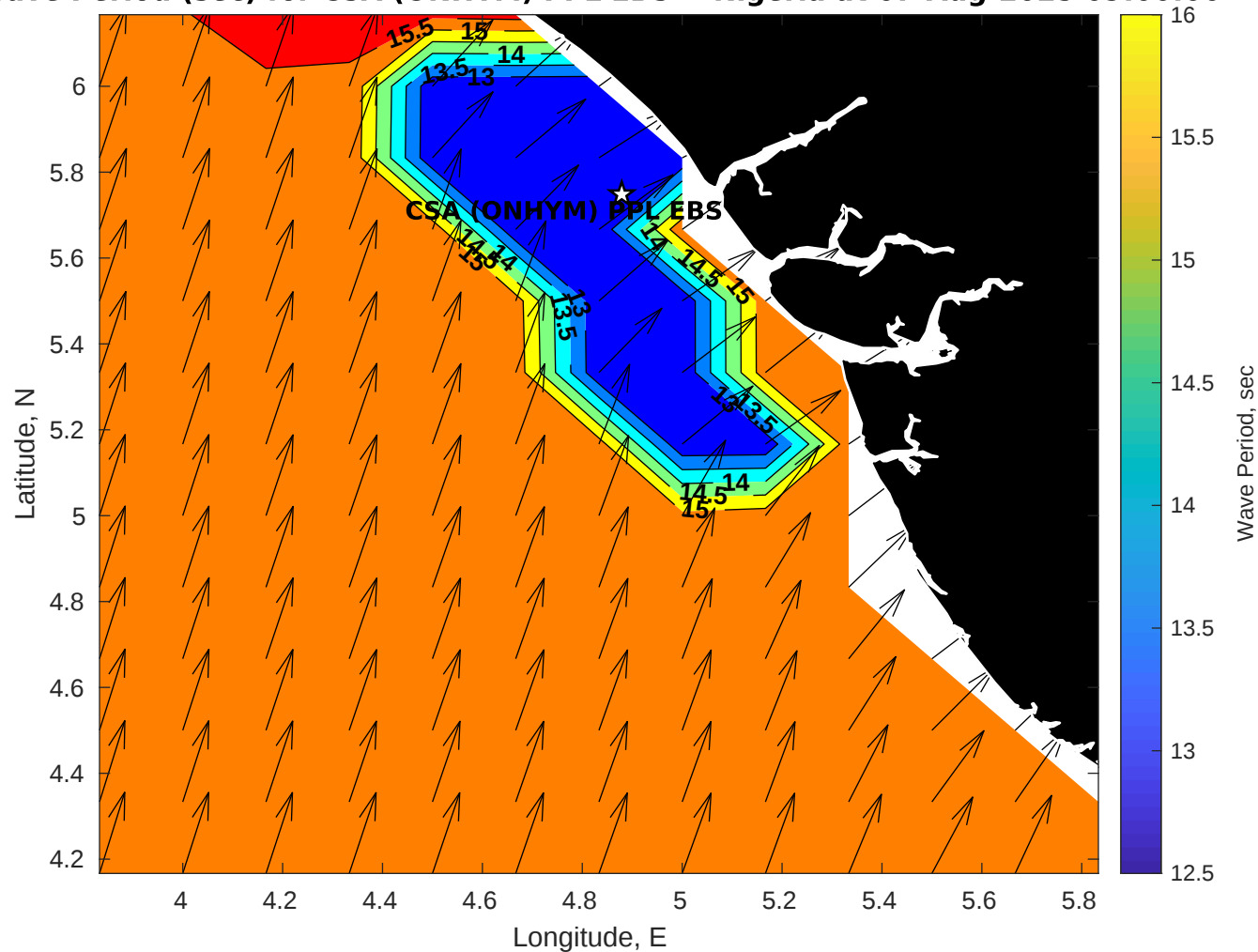
Wave Period (sec) for CSA (ONHYM) PPL EBS - Nigeria at 07-Aug-2025 09:00:00
