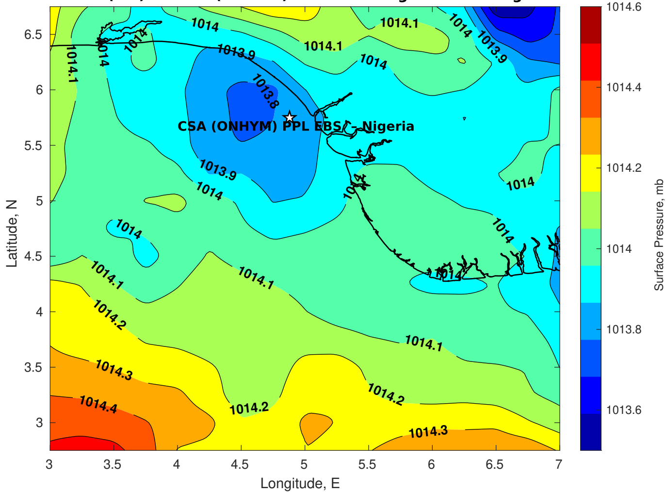
Surface Pressure (mb) for CSA (ONHYM) PPL EBS - Nigeria at 07-Aug-2025 00:00:00
