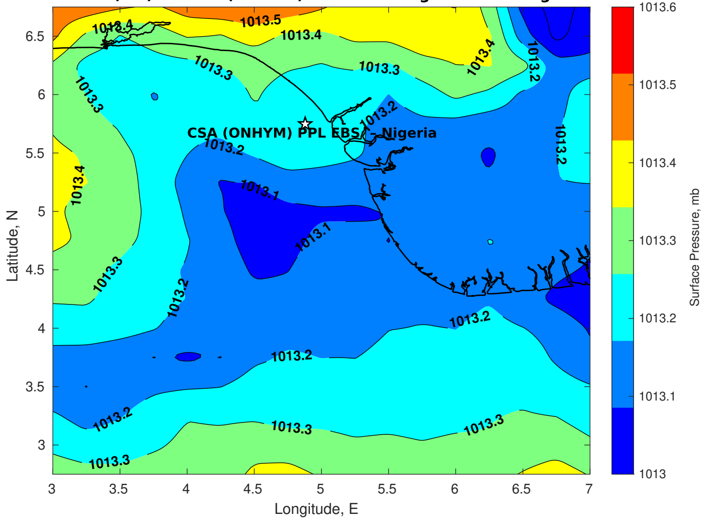
Surface Pressure (mb) for CSA (ONHYM) PPL EBS - Nigeria at 08-Aug-2025 00:00:00
