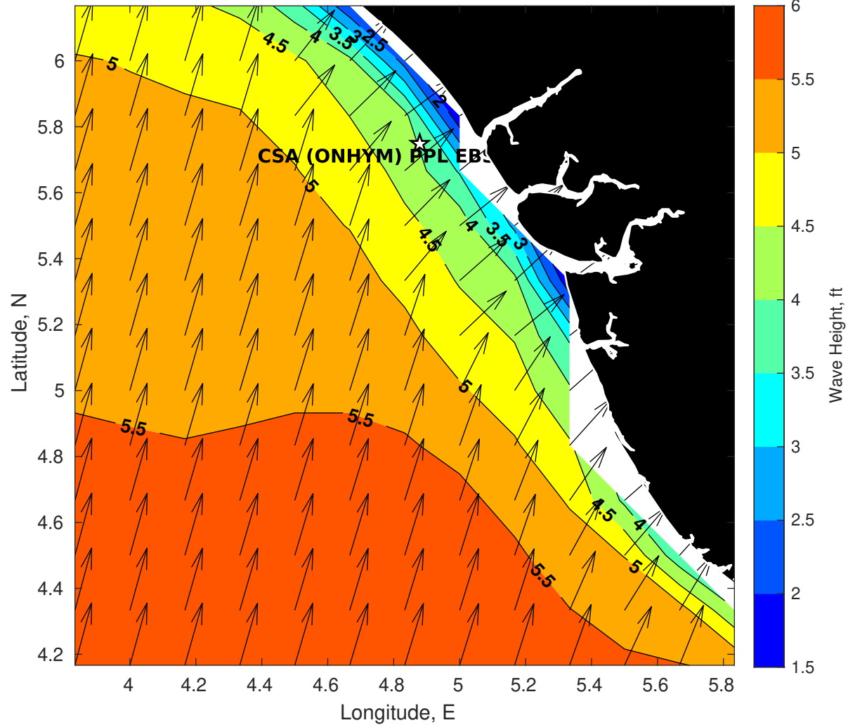
Wave Height (ft) for CSA (ONHYM) PPL EBS - Nigeria at 07-Aug-2025 09:00:00
