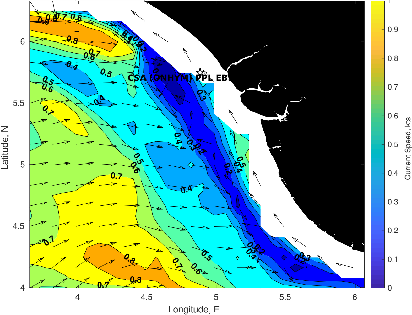
Surface Currents for CSA (ONHYM) PPL EBS - Nigeria at 06-Aug-2025 00:00:00
