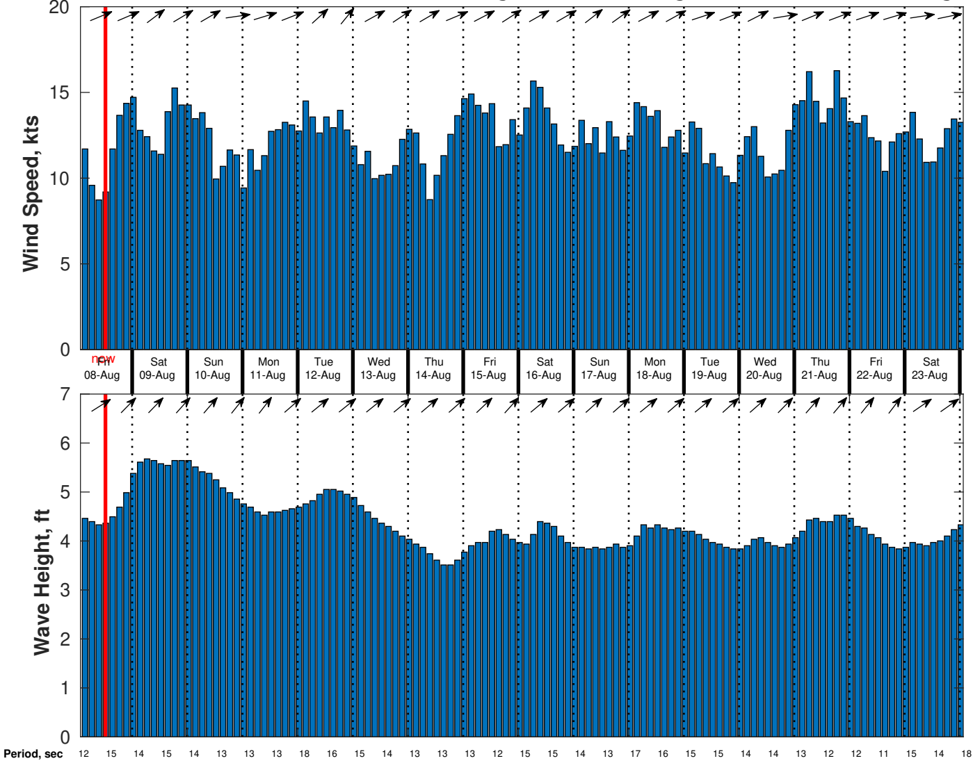
Wind & Wave Forecast for CSA (ONHYM) PPL EBS - Nigeria from 07-Aug-2025 02:00:00 to 23-Aug-2025 02:00:00
