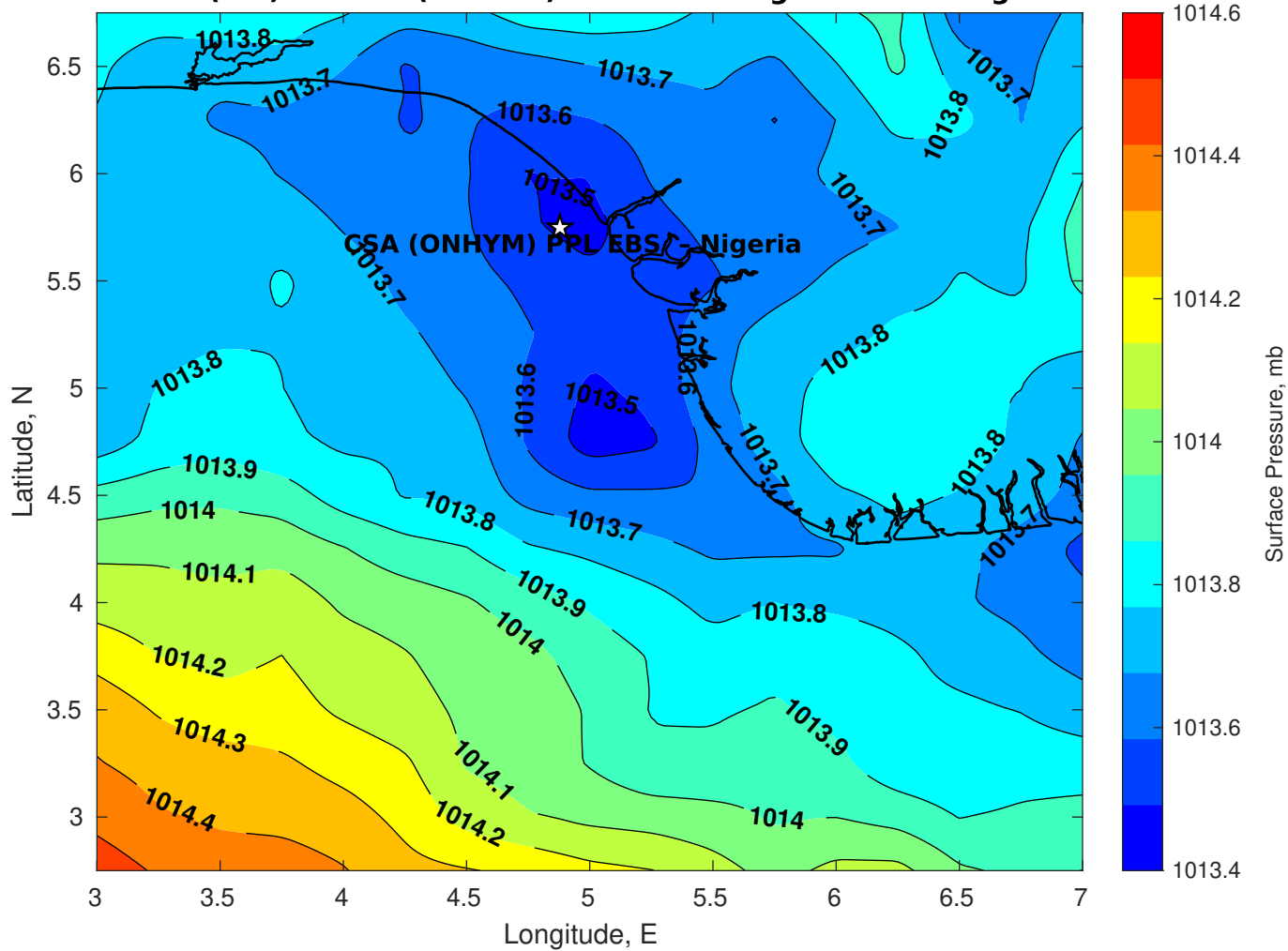
Surface Pressure (mb) for CSA (ONHYM) PPL EBS - Nigeria at 09-Aug-2025 00:00:00
