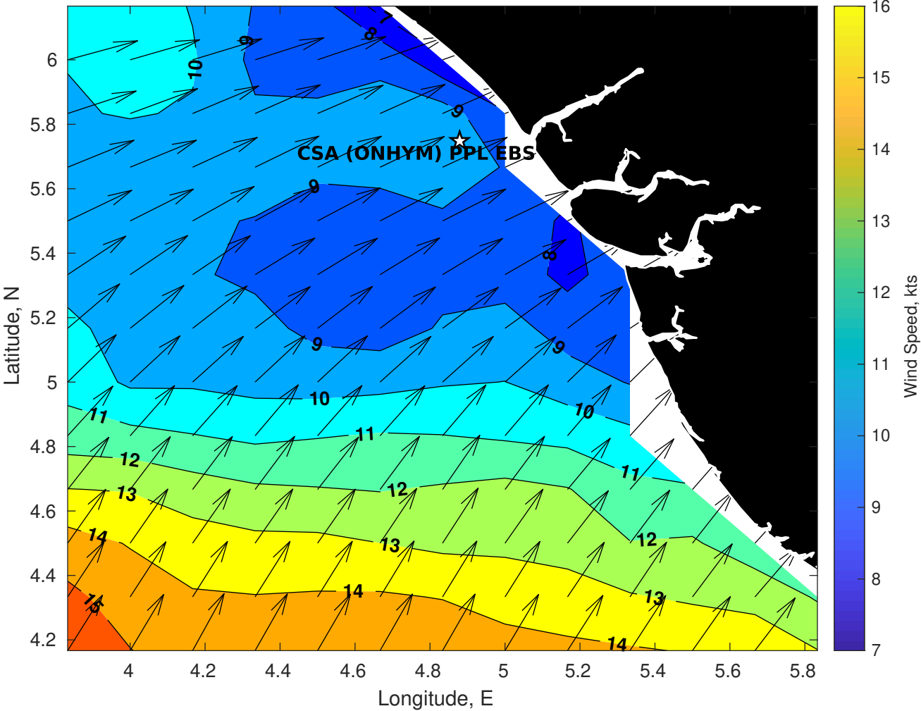
Winds (kts) for CSA (ONHYM) PPL EBS - Nigeria at 07-Aug-2025 09:00:00
