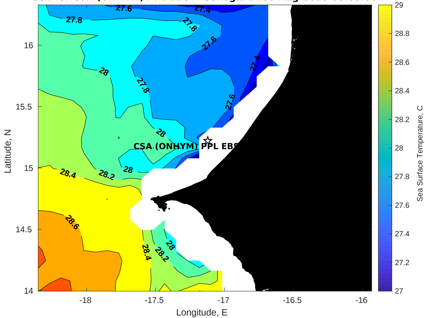
SST for CSA (ONHYM) PPL EBS - Senegal at 06-Aug-2025 00:00:00
