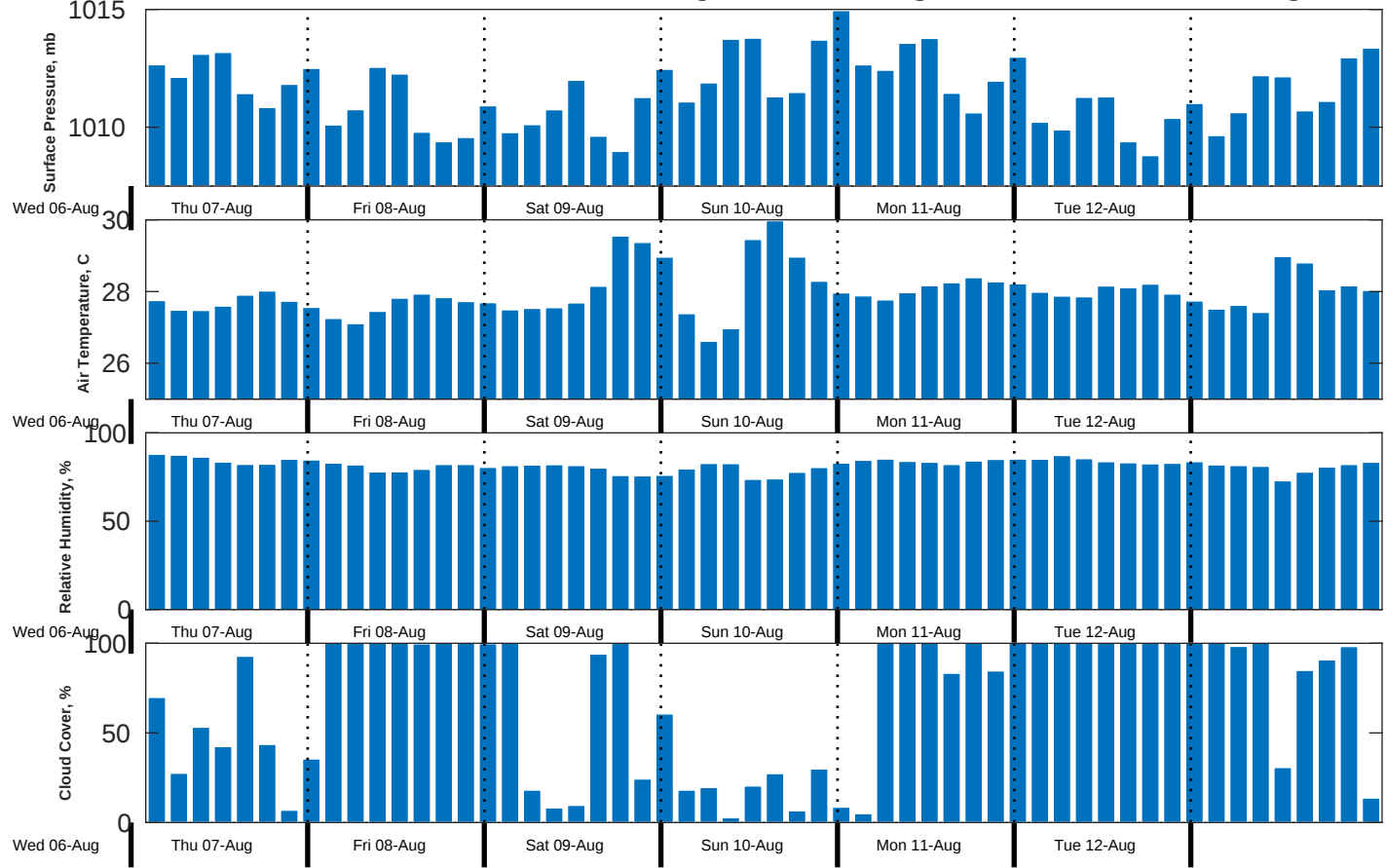
Met Forecast for CSA (ONHYM) PPL EBS - Senegal from 07-Aug-2025 00:00:00 to 14-Aug-2025 00:00:00
