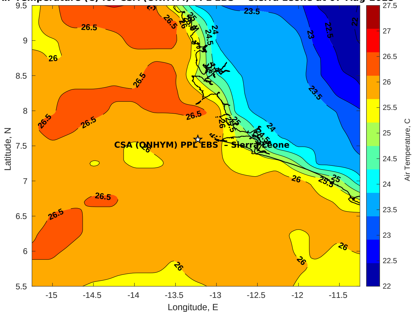
Air Temperature (C) for CSA (ONHYM) PPL EBS - Sierra Leone at 07-Aug-2025
